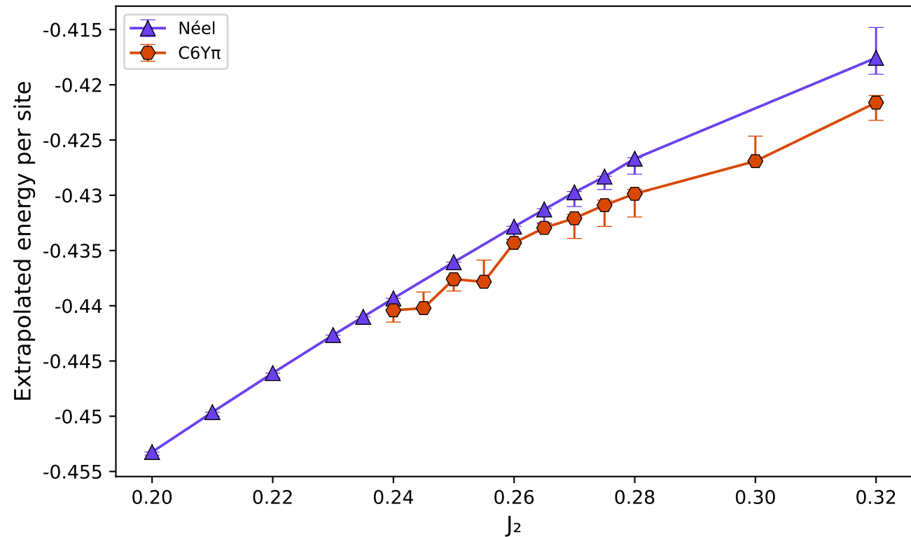
Energy extrapolation: Néel vs C6Y \pi
