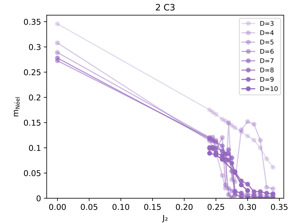
m_{\text{Néel}} vs J_2 — raw D curves
