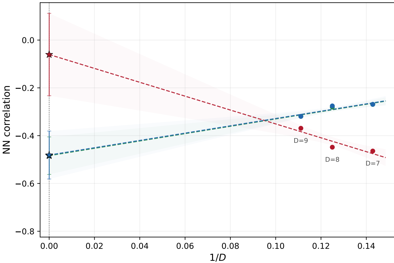
Dimer-plaquette seed, J_2 = 0.265
