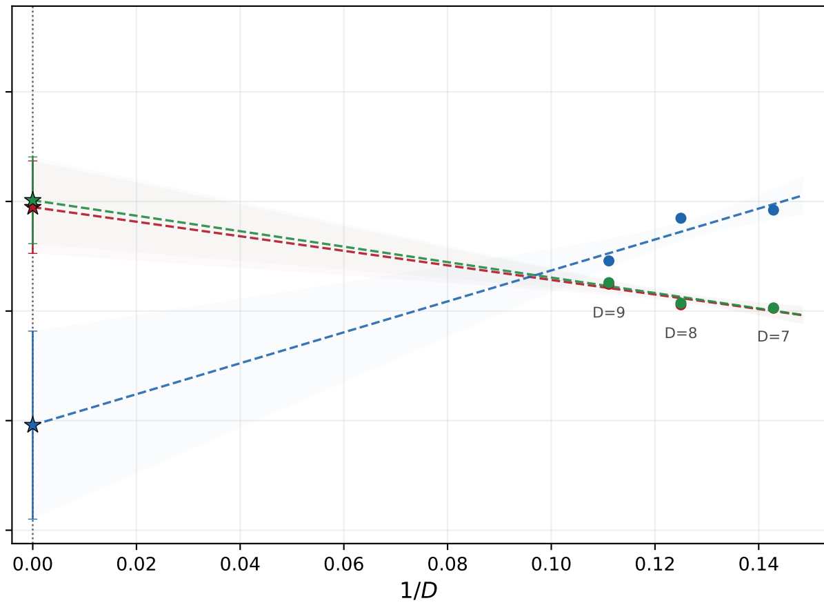
Plaquette seed, J_2 = 0.265
