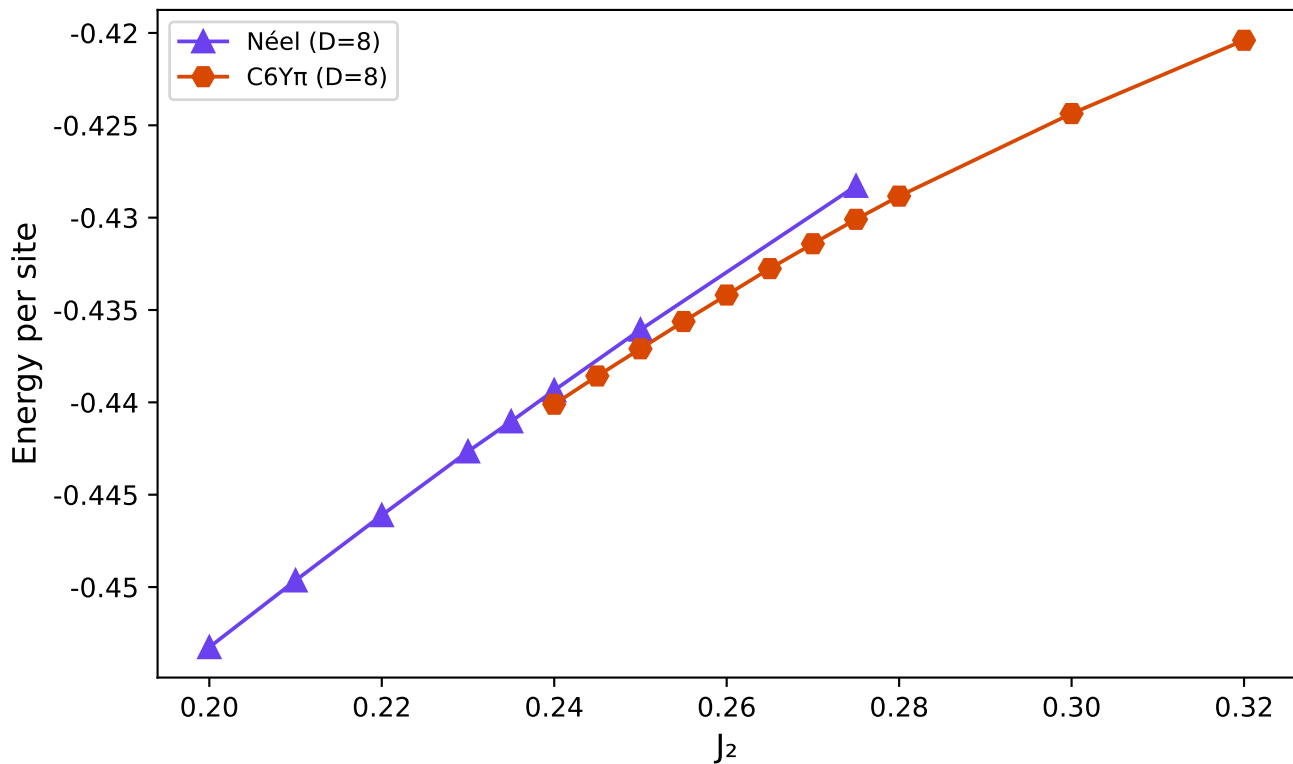
Energy: Néel ( D=8 ) vs C6Y \pi ( D=8 )
