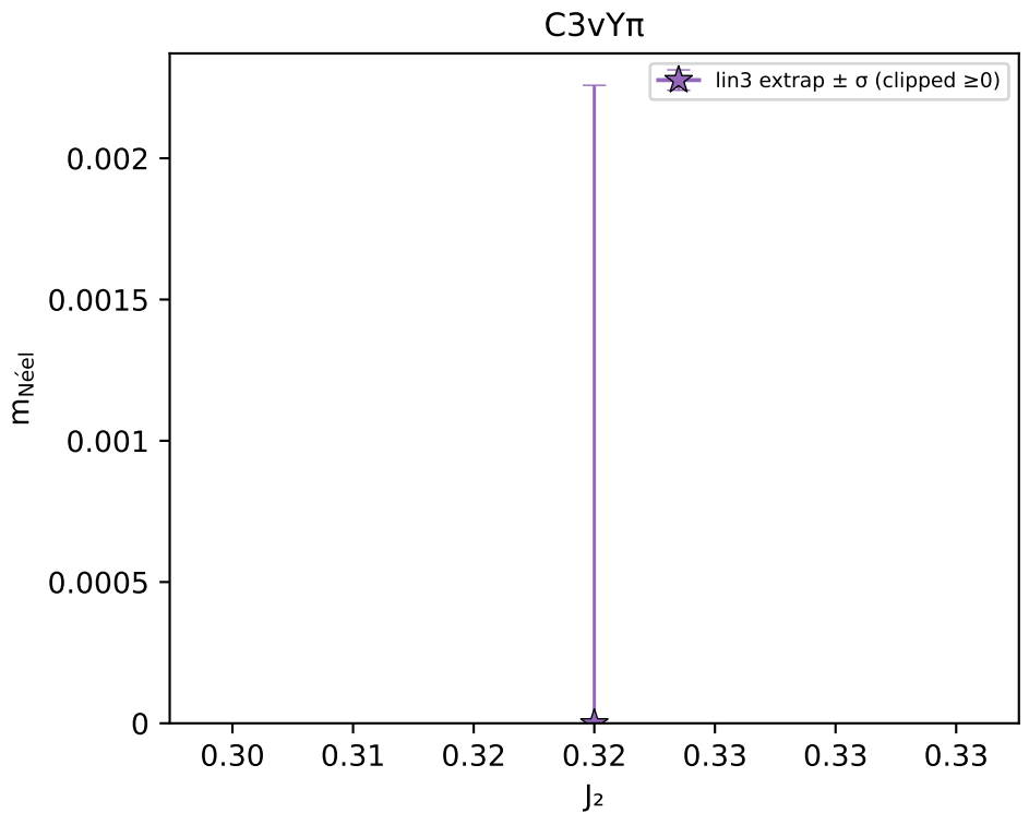
m_{\text{Néel}} vs J_2 — lin3 extrapolated \pm \sigma
