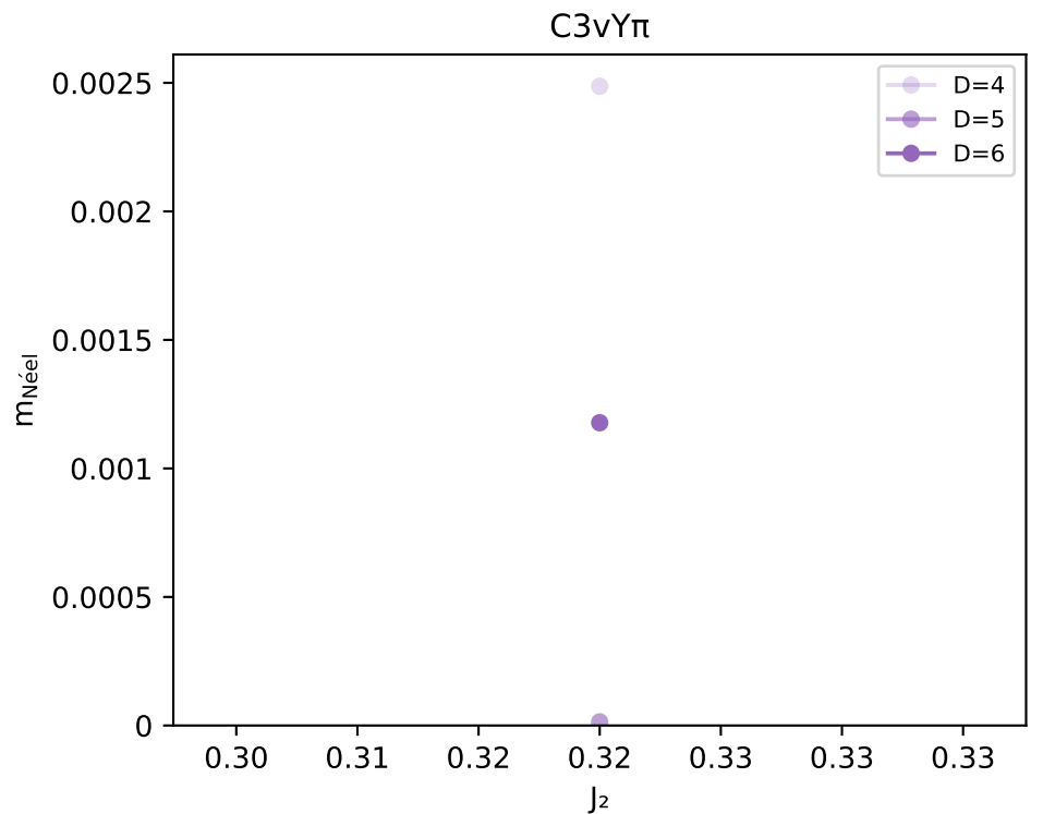
m_{\text{Néel}} vs J_2 — raw D curves
