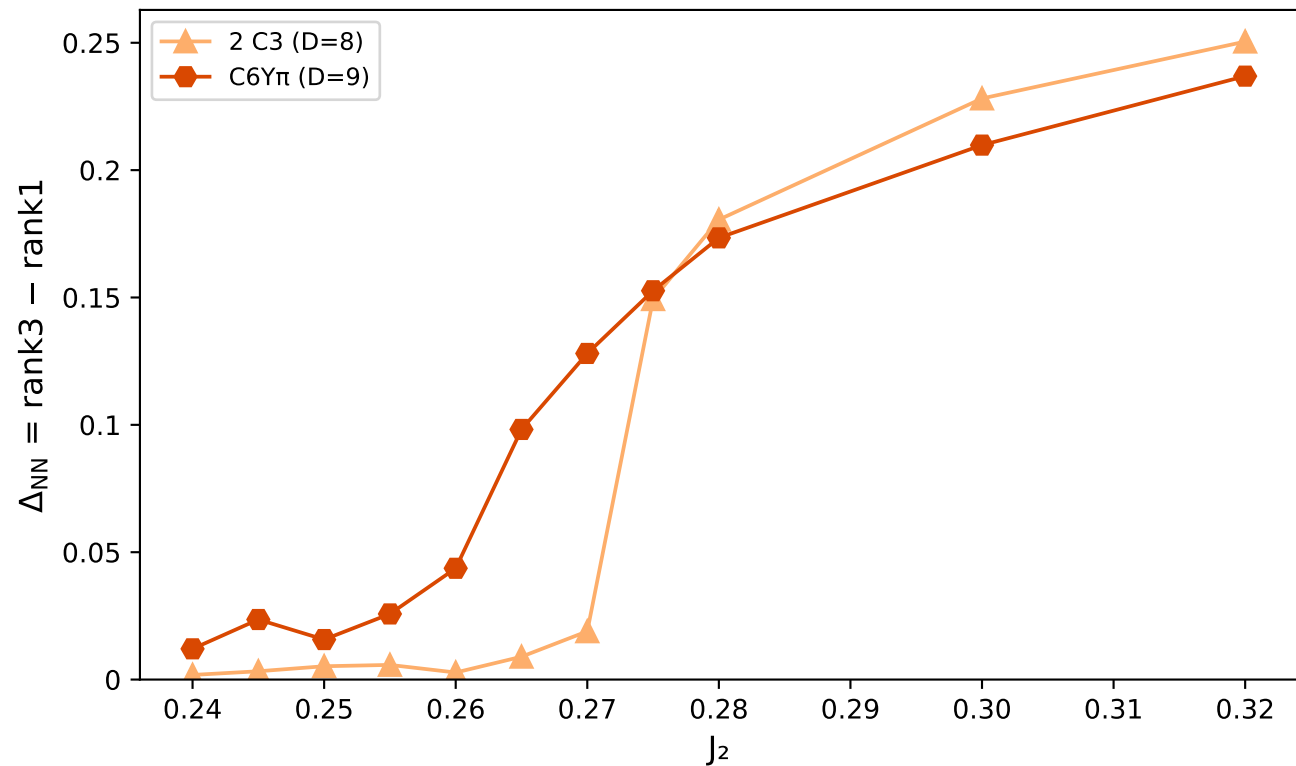
NN bond splitting: 2C3 (D=8) vs C6Y \pi (D=9)
