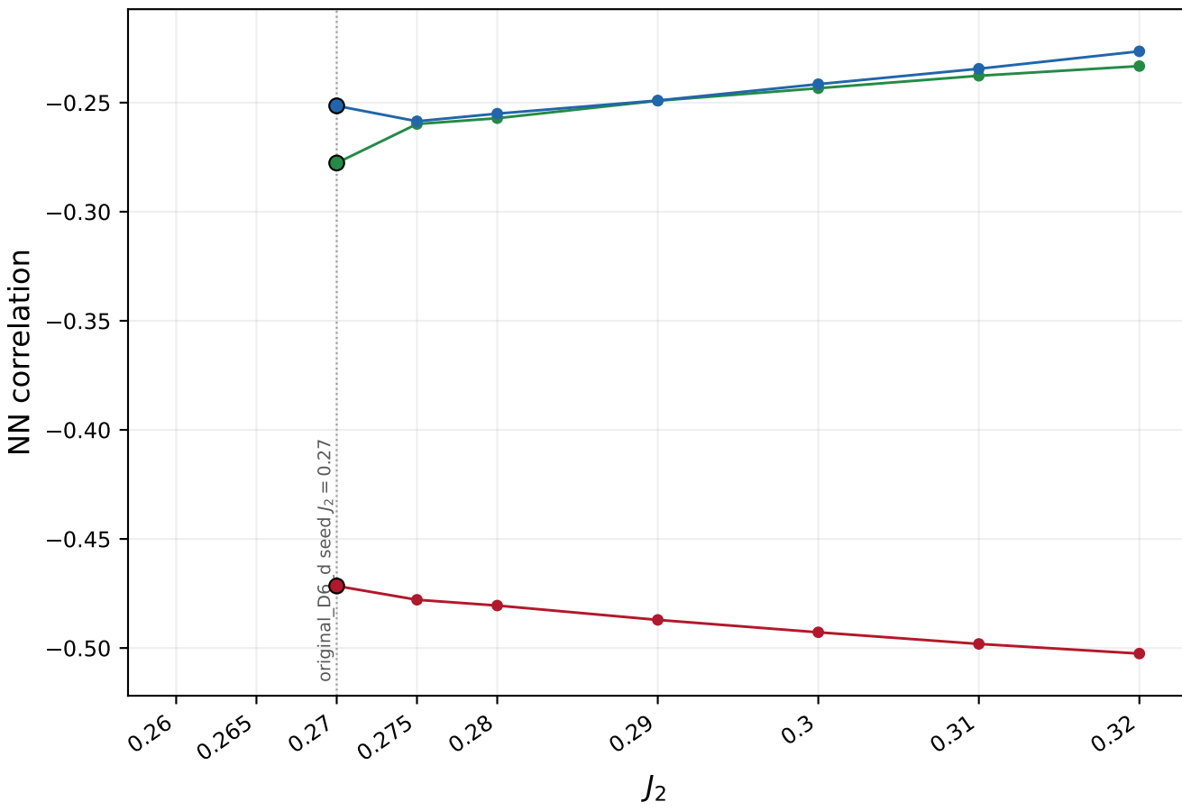
Dimer-plaquette seed, D = 6
