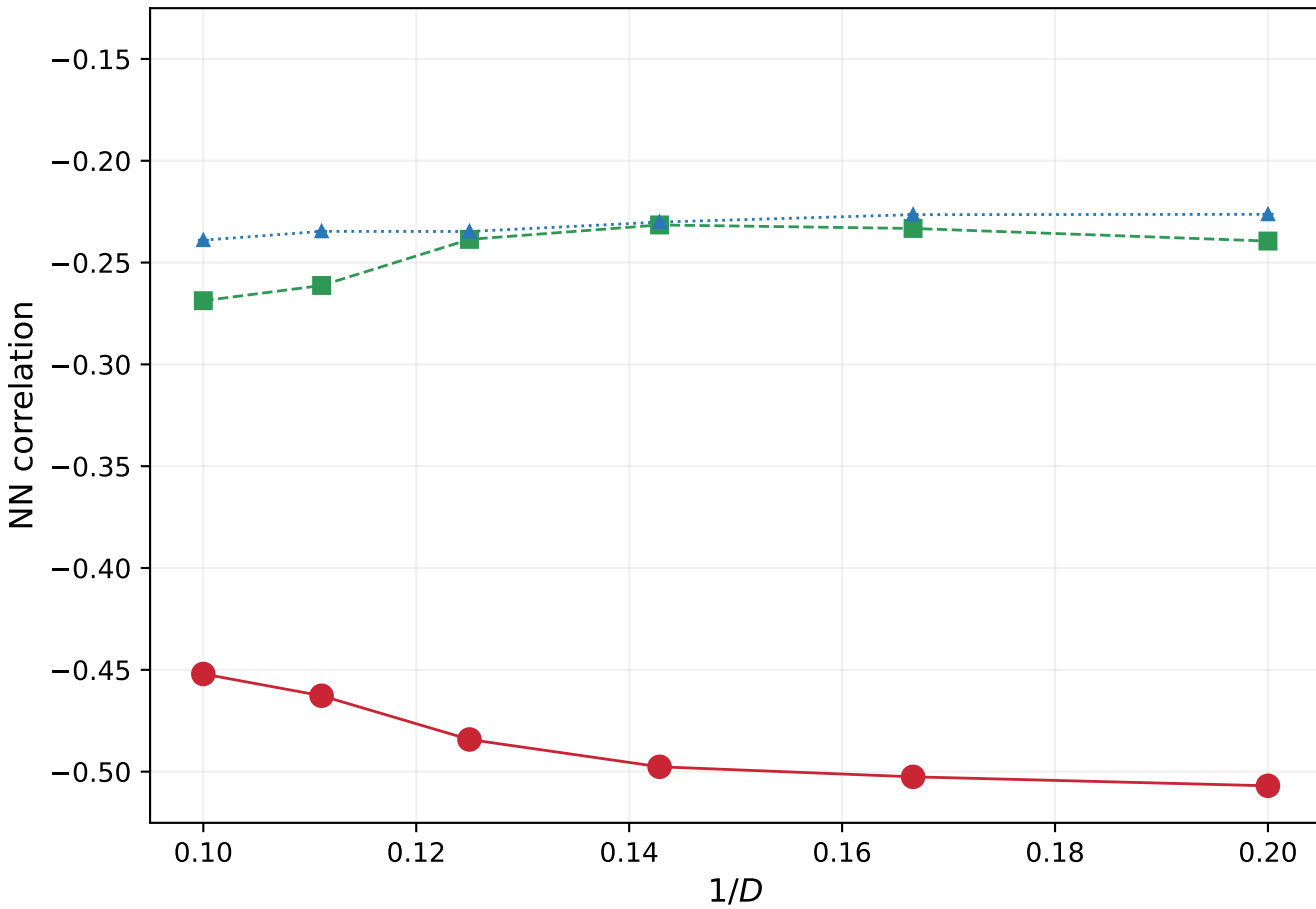
Dimer-plaquette sector, J_2 = 0.32
