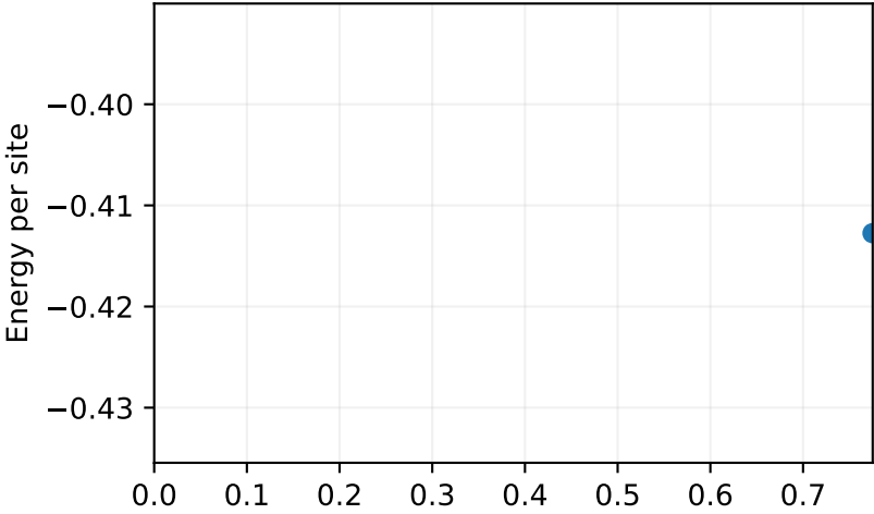
observables vs 1/\xi
