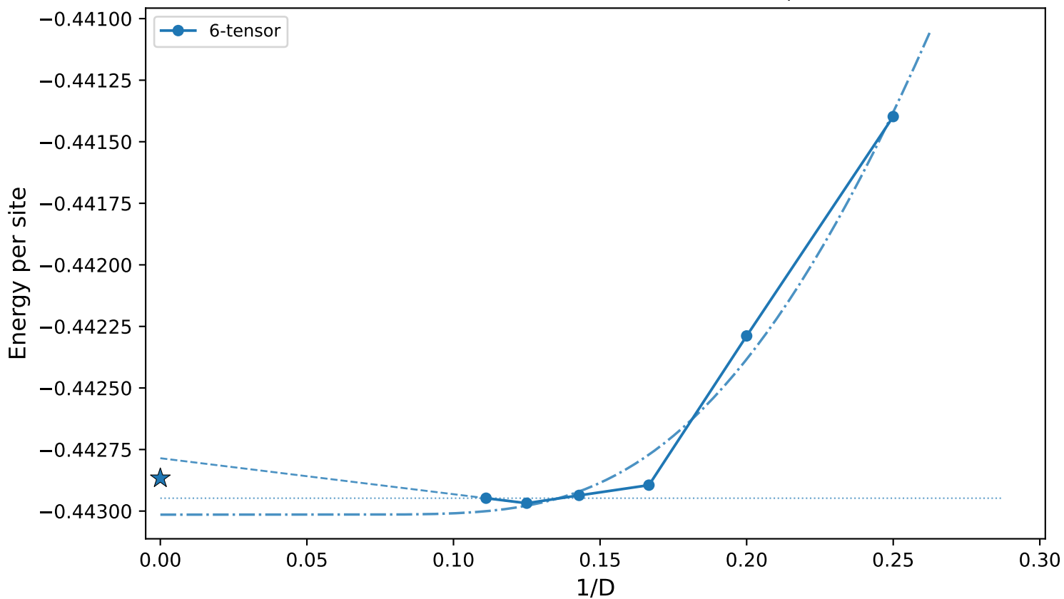
J_2=0.23 - Energy vs 1/D (6-tensor) (dotted=horizontal, dashed=linear last-2, dash-dot=exp all- D s, \star=E_0 )
