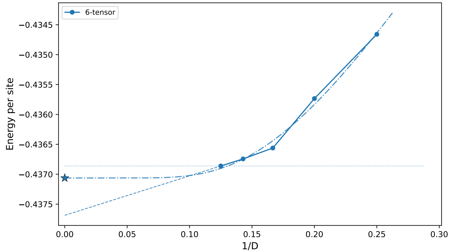
J_2=0.25 - Energy vs 1/D (6-tensor) (dotted=horizontal, dashed=linear last-2, dash-dot=exp all-Ds, ★= E_0 )
