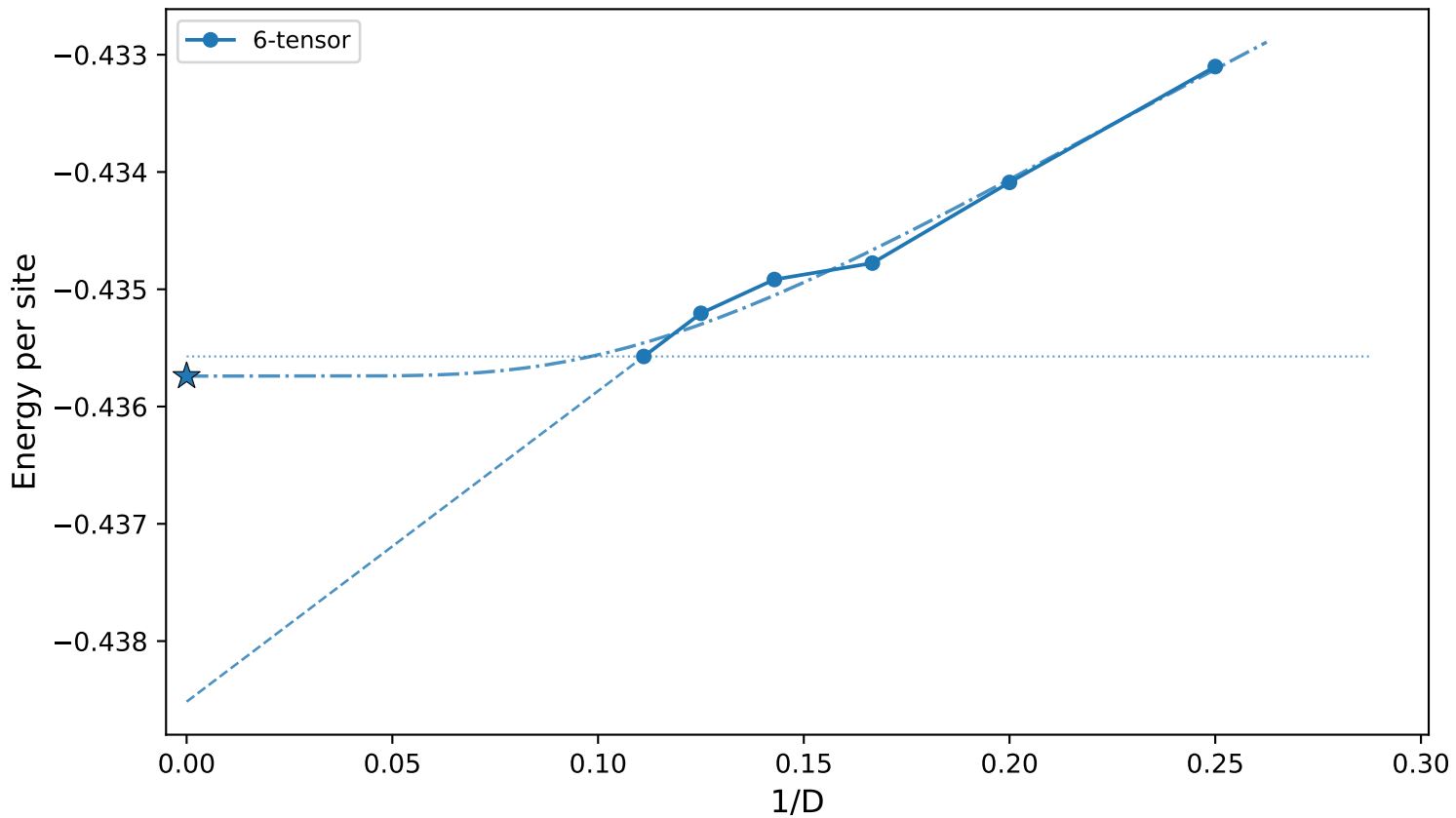
J_2=0.255 - Energy vs 1/D (6-tensor) (dotted=horizontal, dashed=linear last-2, dash-dot=exp all- D s, ★= E_0 )
