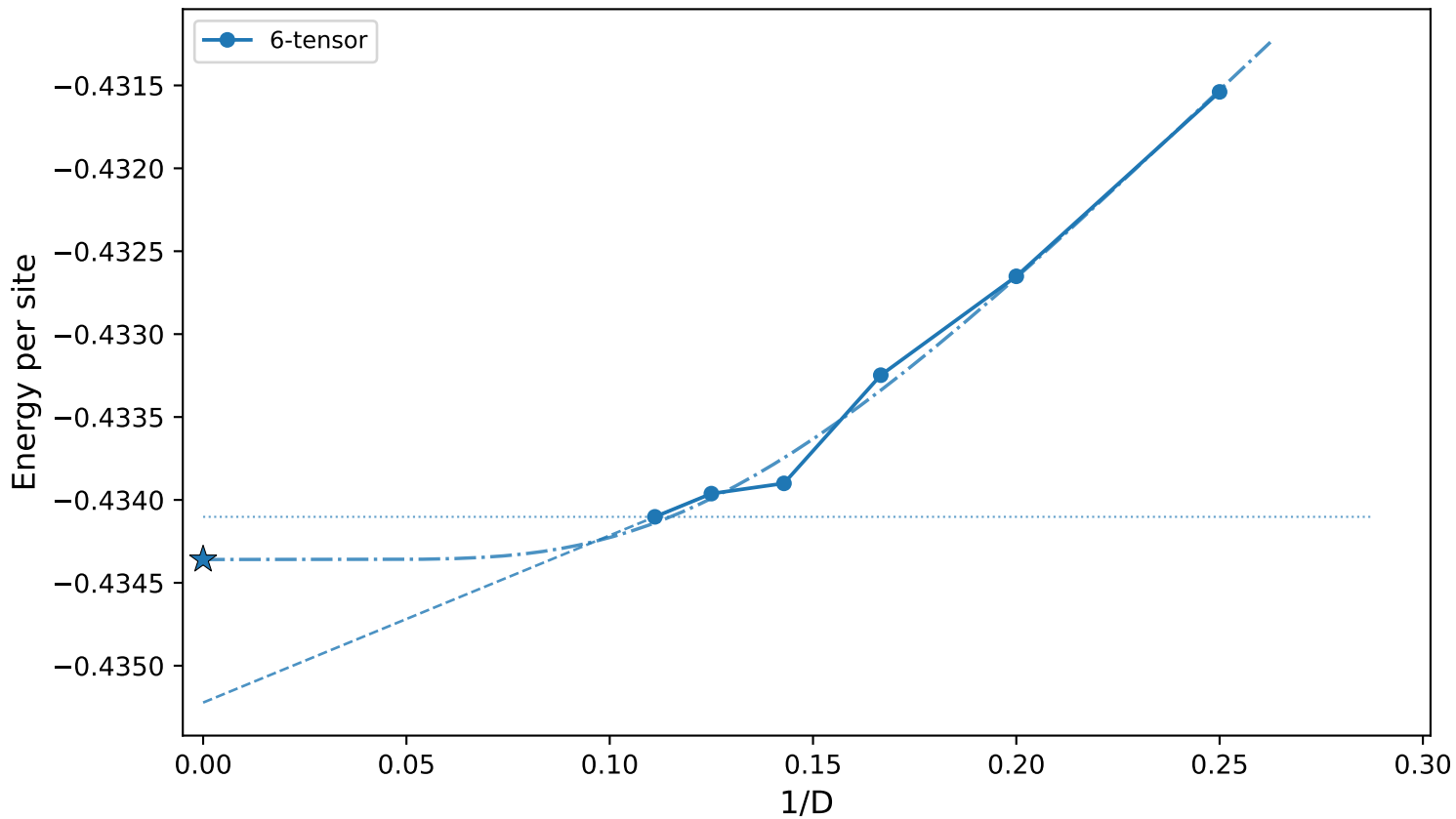
J_2=0.26 - Energy vs 1/D (6-tensor) (dotted=horizontal, dashed=linear last-2, dash-dot=exp all- D s, \star=E_0 )
