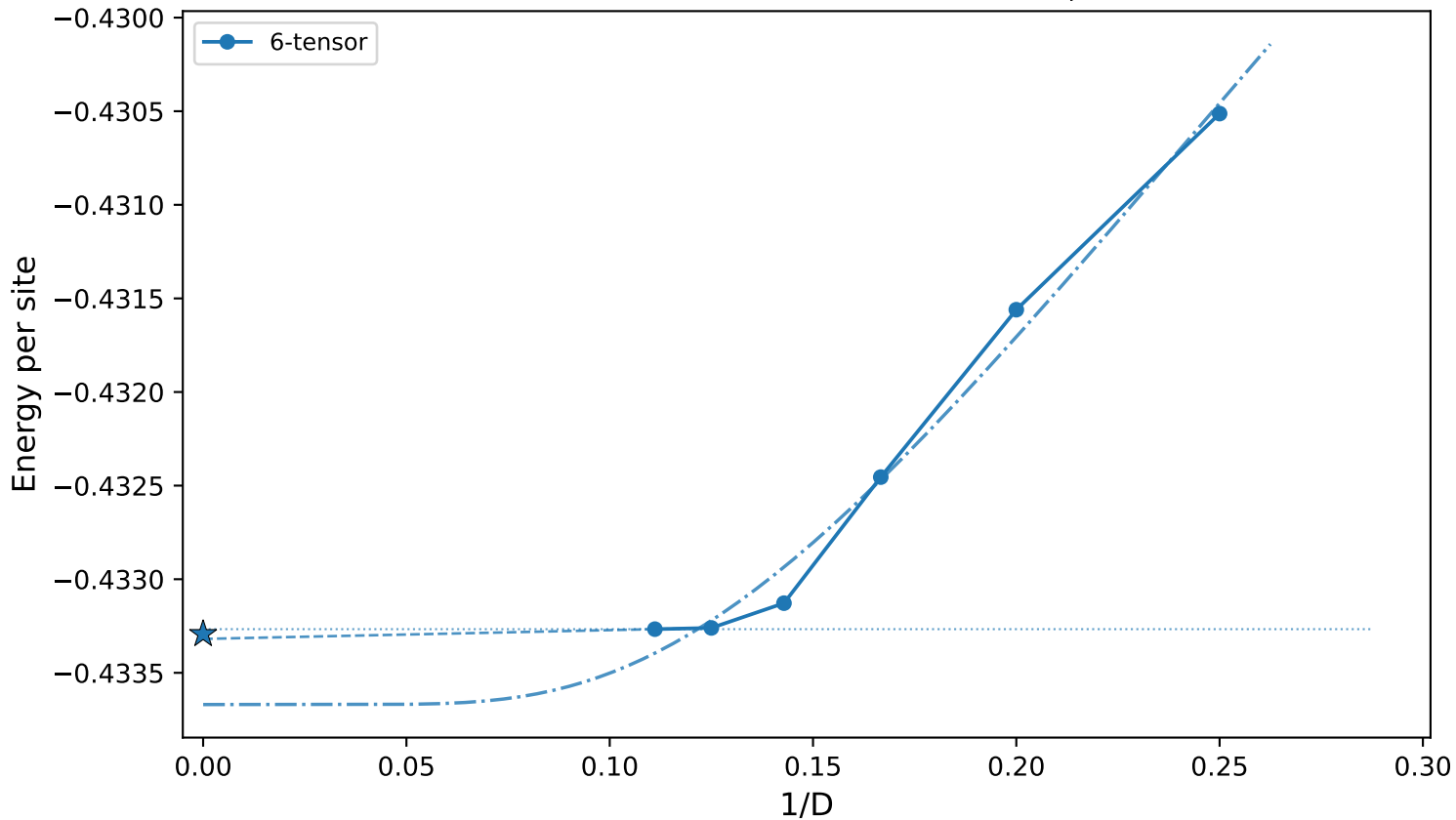
J2=0.263 - Energy vs 1/D (6-tensor) (dotted=horizontal, dashed=linear last-2, dash-dot=exp all-Ds, ★=E 0 )
