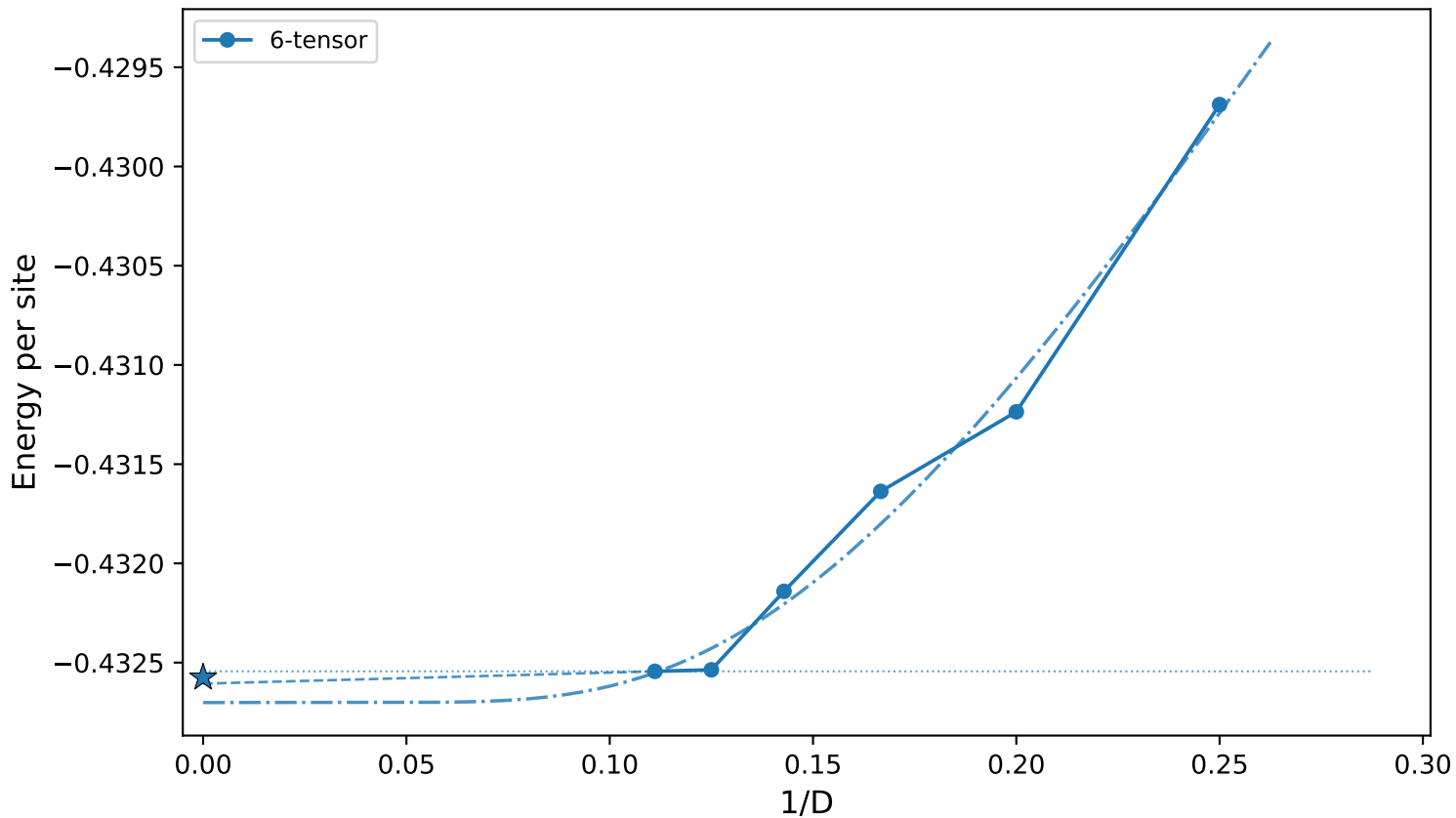
J_2=0.266 - Energy vs 1/D (6-tensor) (dotted=horizontal, dashed=linear last-2, dash-dot=exp all- D s, \star=E_0 )
