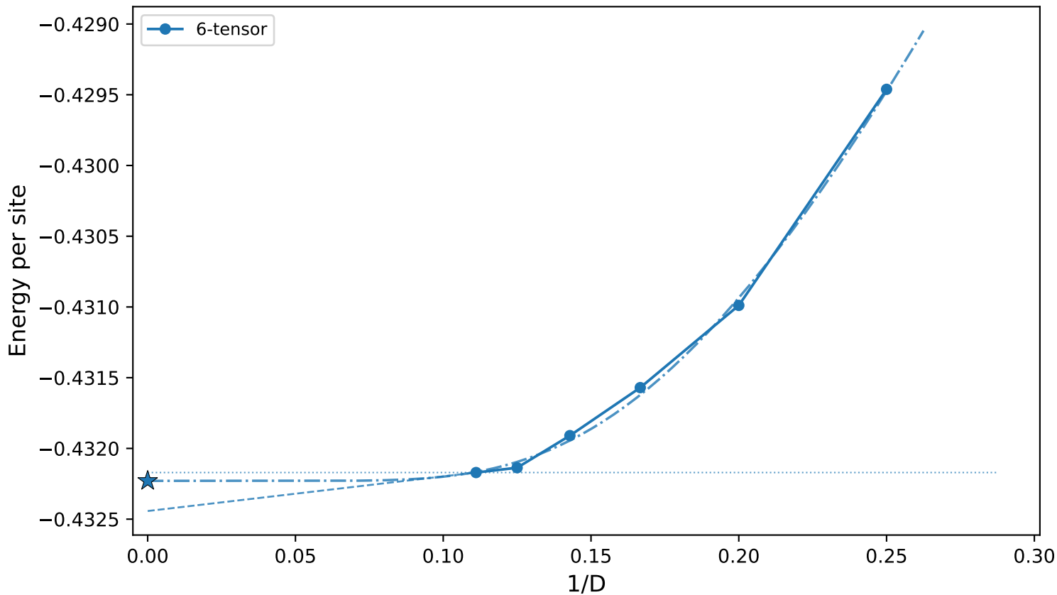
J_2=0.267 - Energy vs 1/D (6-tensor) (dotted=horizontal, dashed=linear last-2, dash-dot=exp all- D s, \star=E_0 )
