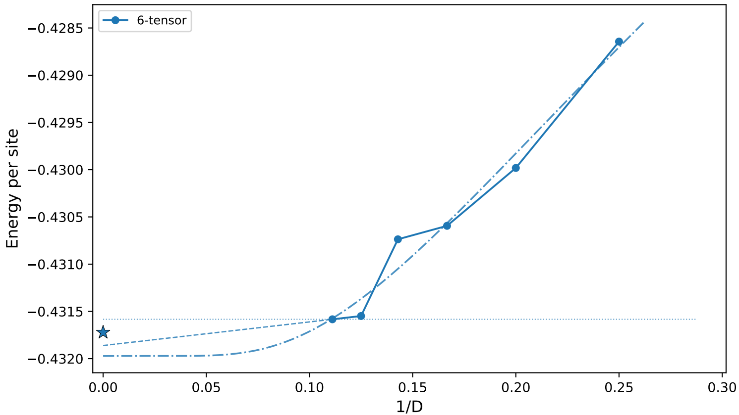
J_2=0.269 - Energy vs 1/D (6-tensor) (dotted=horizontal, dashed=linear last-2, dash-dot=exp all- D s, \star=E_0 )
