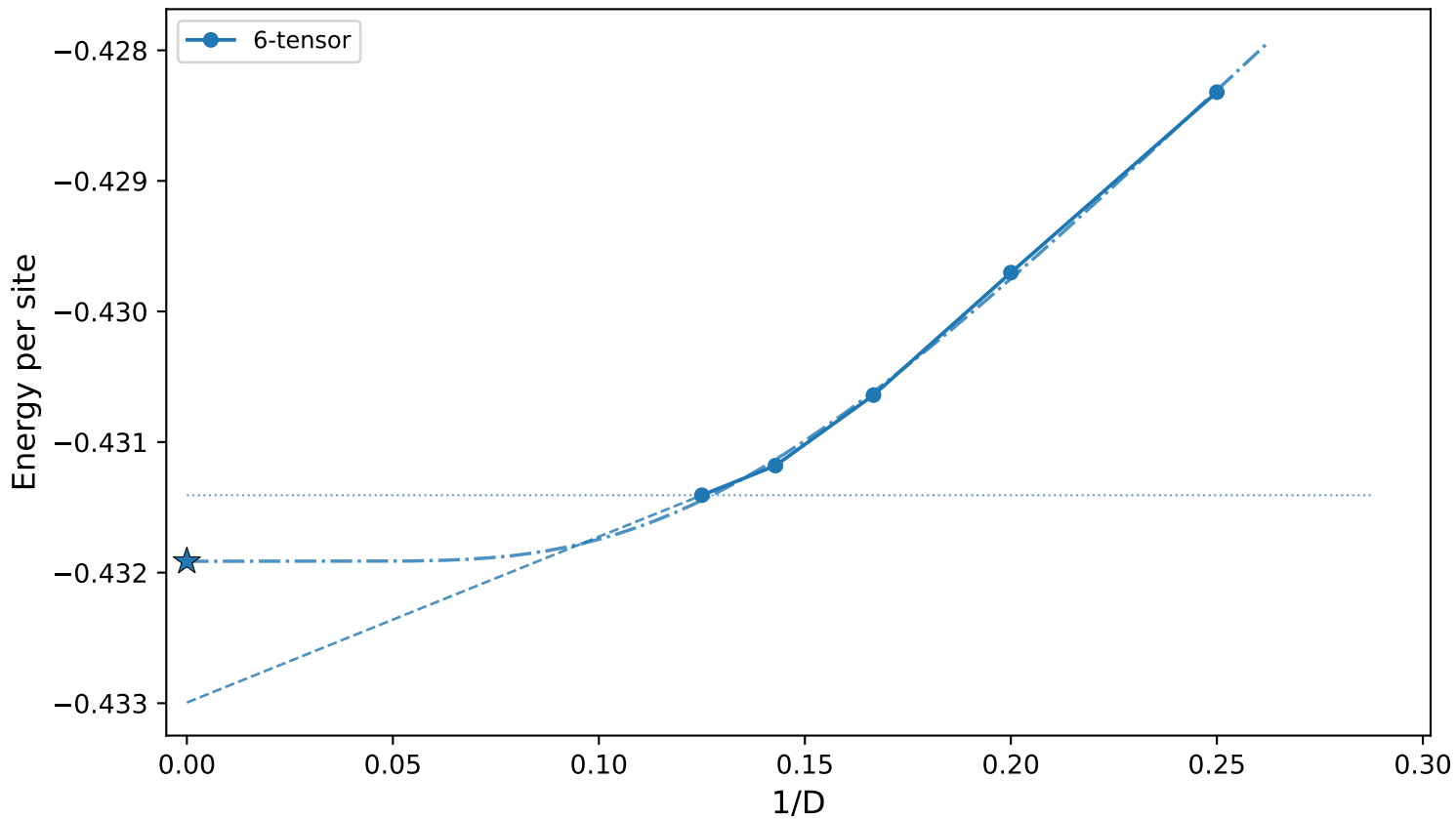
J_2=0.27 - Energy vs 1/D (6-tensor) (dotted=horizontal, dashed=linear last-2, dash-dot=exp all- D s, \star=E_0 )
