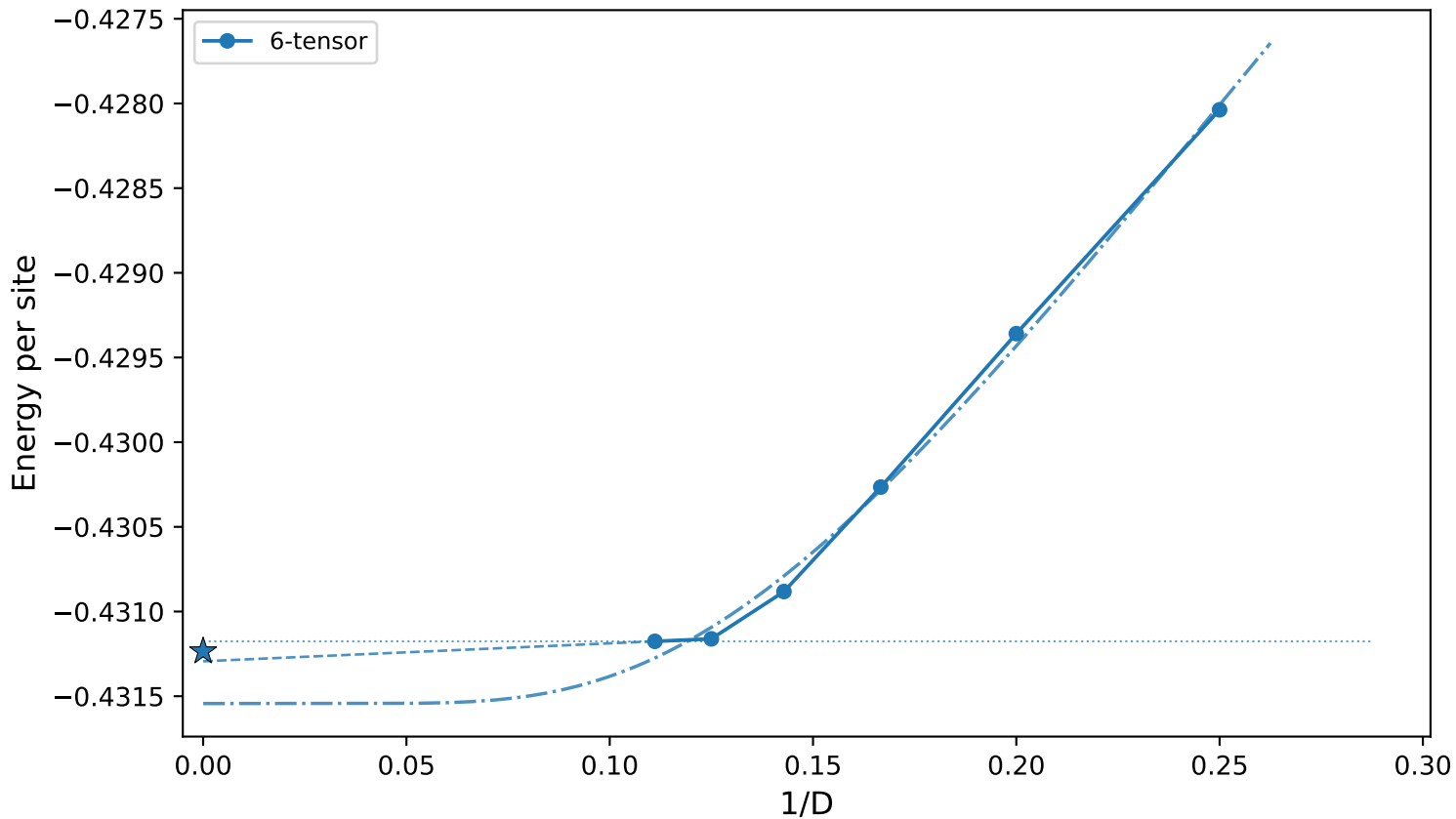
J_2=0.271 - Energy vs 1/D (6-tensor) (dotted=horizontal, dashed=linear last-2, dash-dot=exp all-Ds, ★= E_0 )
