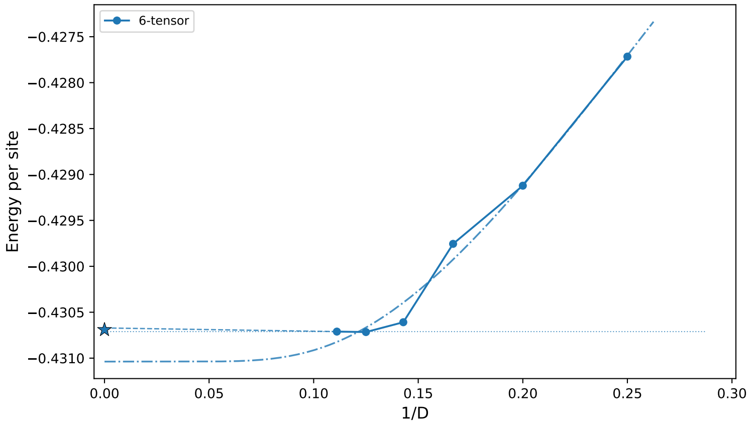
J_2=0.272 - Energy vs 1/D (6-tensor) (dotted=horizontal, dashed=linear last-2, dash-dot=exp all-Ds, ★= E_0 )
