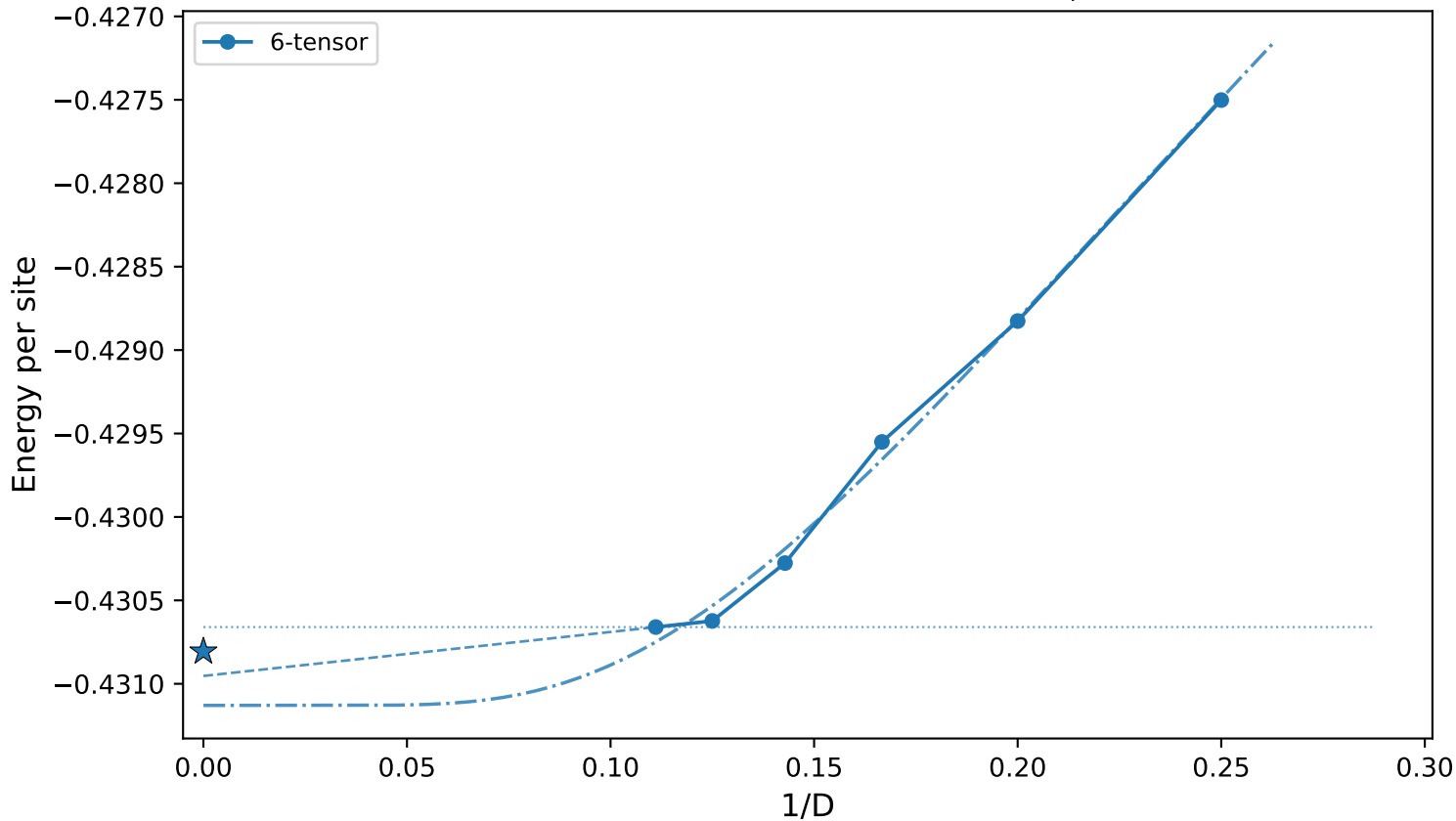
J_2=0.273 - Energy vs 1/D (6-tensor) (dotted=horizontal, dashed=linear last-2, dash-dot=exp all- D s, ★= E_0 )
