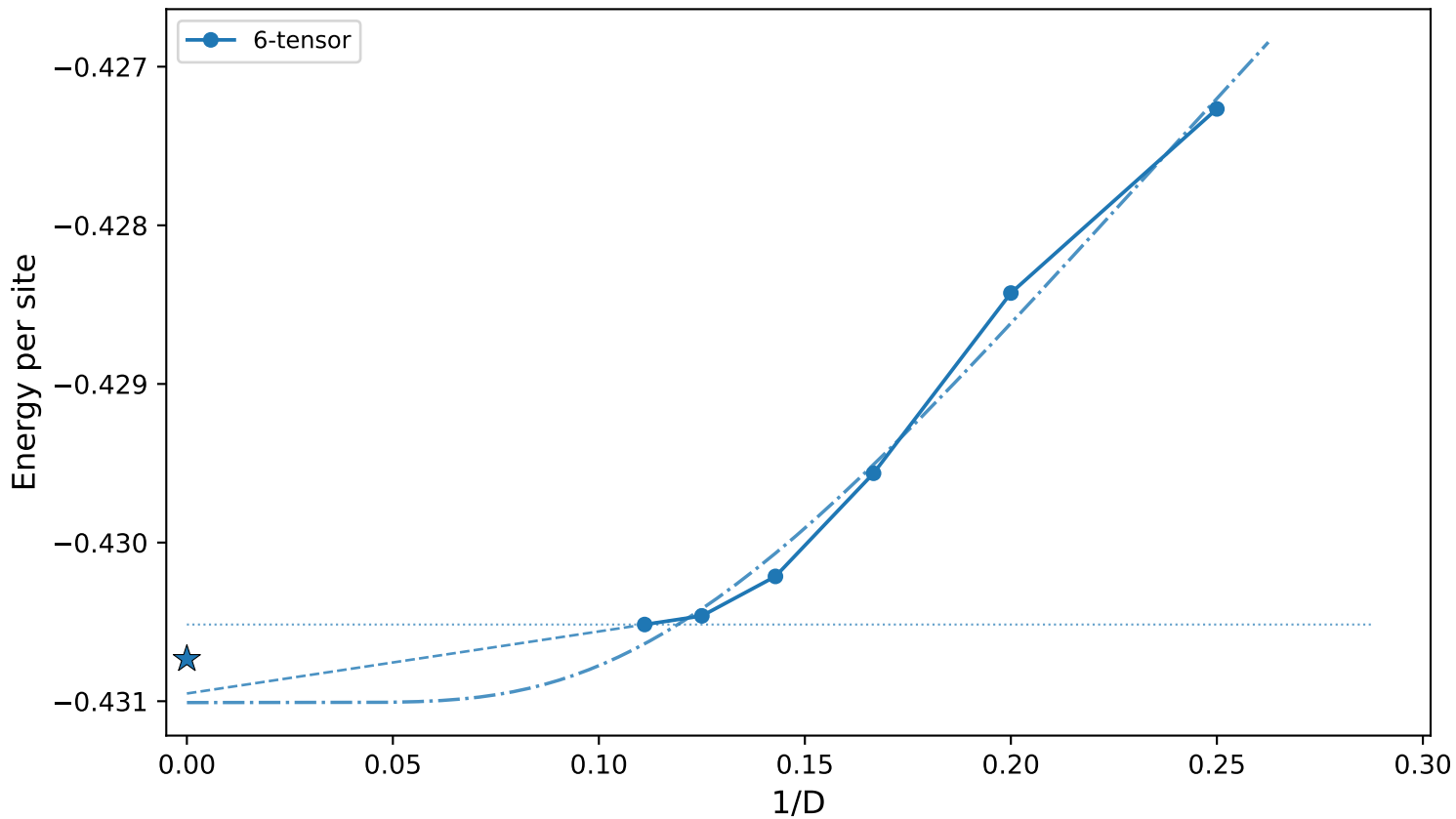
J_2=0.274 - Energy vs 1/D (6-tensor) (dotted=horizontal, dashed=linear last-2, dash-dot=exp all- D s, \star=E_0 )
