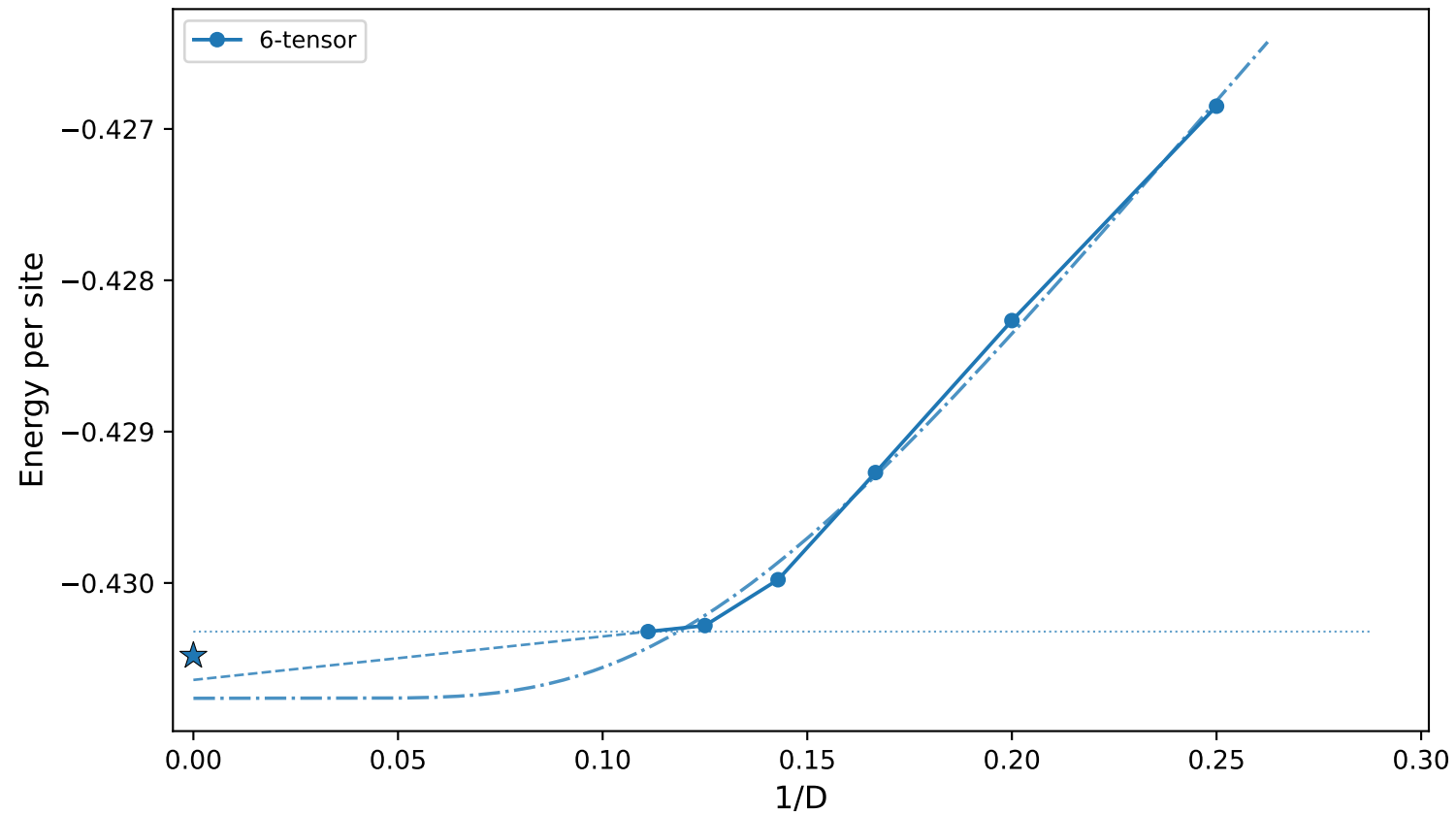
J_2=0.275 - Energy vs 1/D (6-tensor) (dotted=horizontal, dashed=linear last-2, dash-dot=exp all-Ds, ★= E_0 )
