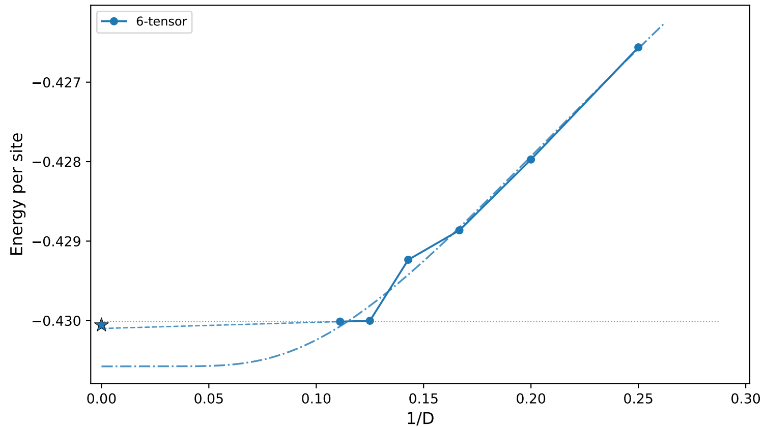
J_2=0.276 - Energy vs 1/D (6-tensor) (dotted=horizontal, dashed=linear last-2, dash-dot=exp all- D s, \star=E_0 )
