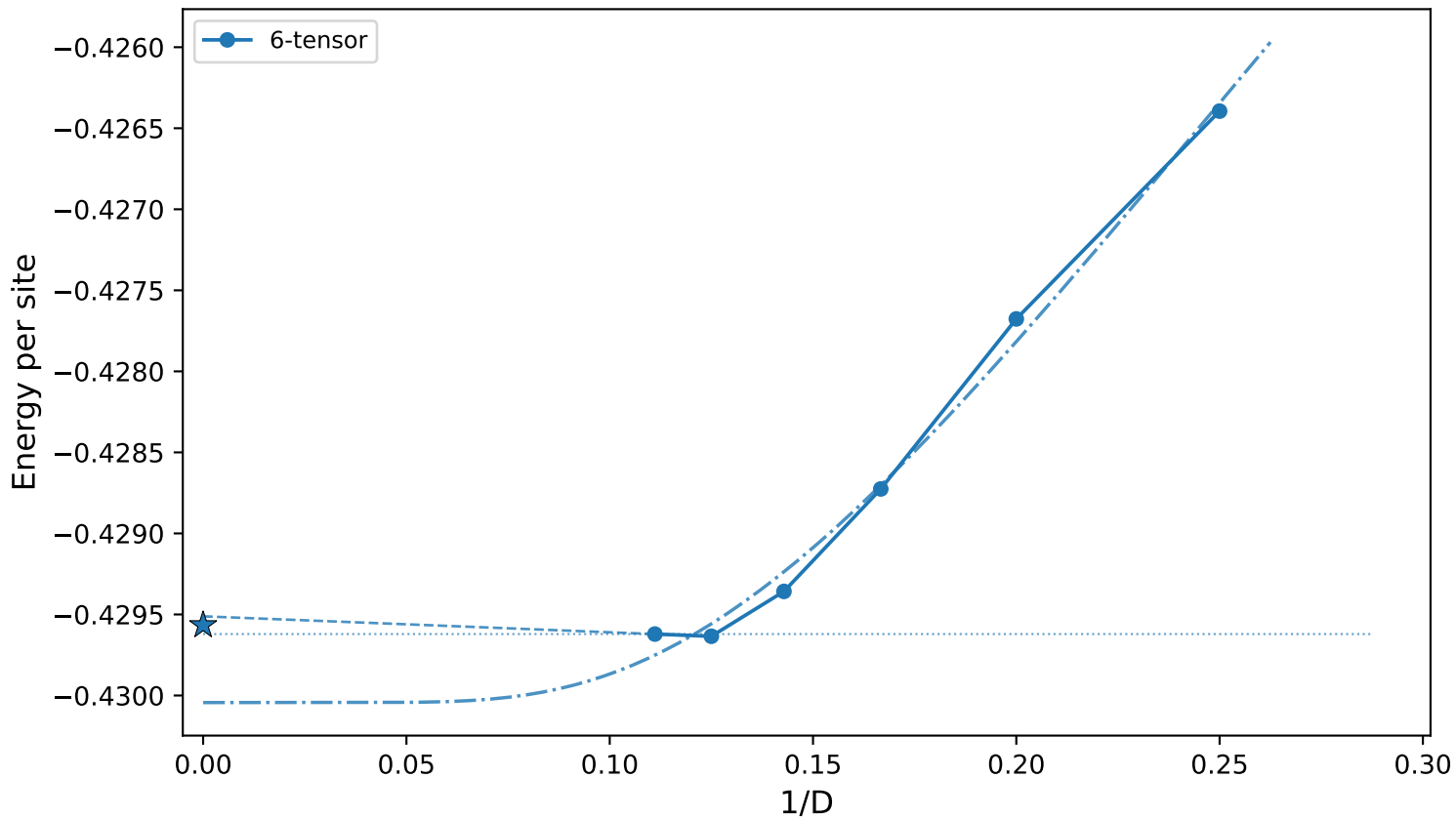
J_2=0.277 - Energy vs 1/D (6-tensor) (dotted=horizontal, dashed=linear last-2, dash-dot=exp all- D s, \star=E_0 )
