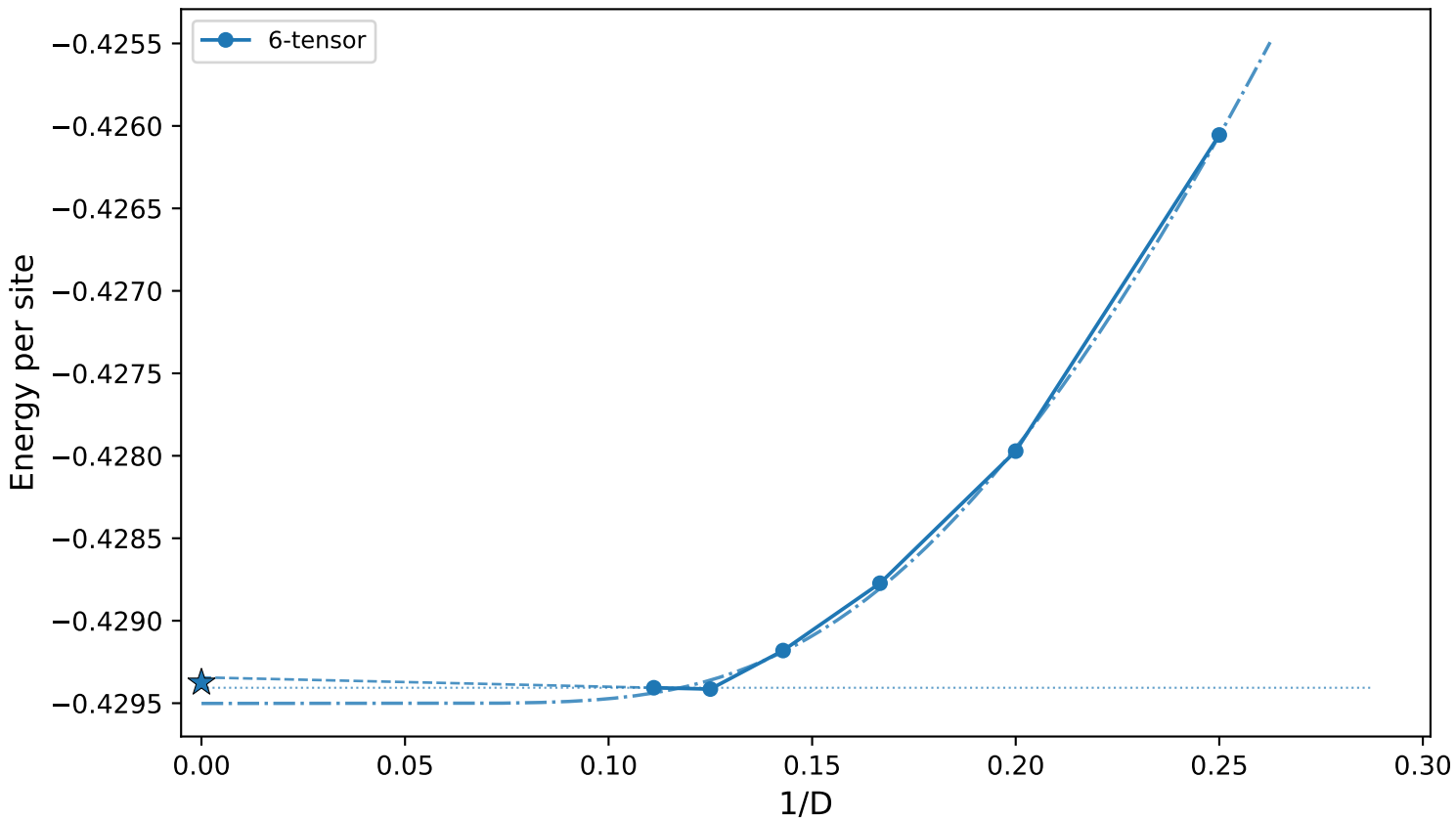
J_2=0.278 - Energy vs 1/D (6-tensor) (dotted=horizontal, dashed=linear last-2, dash-dot=exp all- D s, \star=E_0 )
