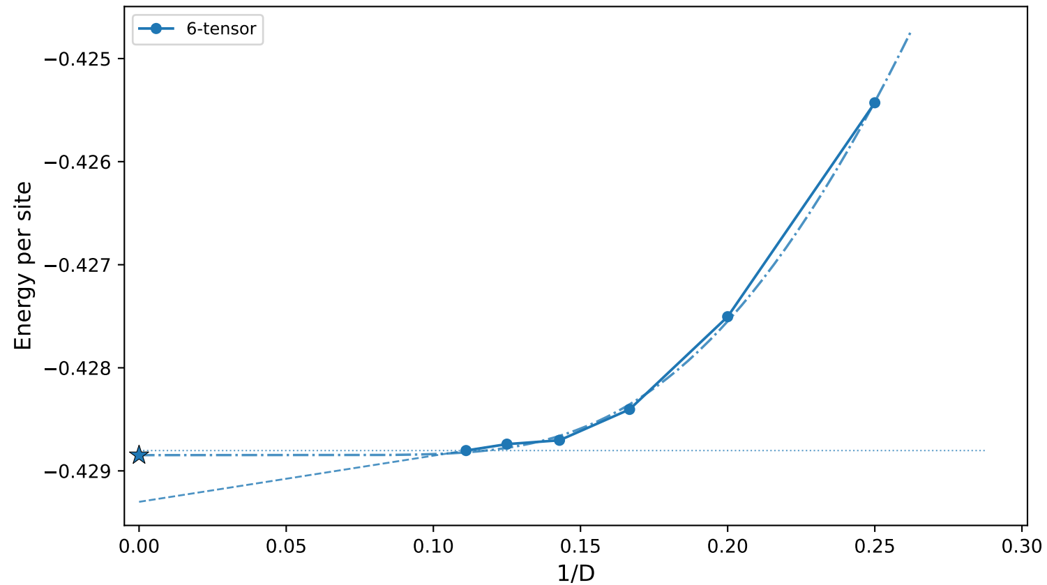
J_2=0.28 - Energy vs 1/D (6-tensor) (dotted=horizontal, dashed=linear last-2, dash-dot=exp all- D s, \star=E_0 )
