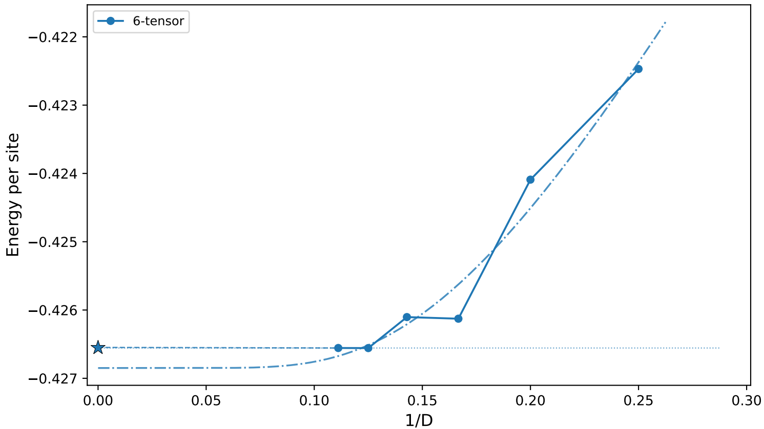
J_2=0.29 - Energy vs 1/D (6-tensor) (dotted=horizontal, dashed=linear last-2, dash-dot=exp all- D s, \star=E_0 )
