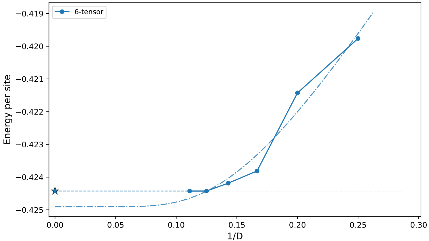
J_2=0.30 - Energy vs 1/D (6-tensor) (dotted=horizontal, dashed=linear last-2, dash-dot=exp all- D s, \star=E_0 )
