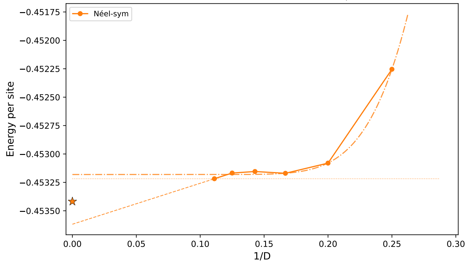
J_2=0.20 - Energy vs 1/D (Néel-sym) (dotted=horizontal, dashed=linear last-2, dash-dot=exp all- D s, ★= E_0 )
