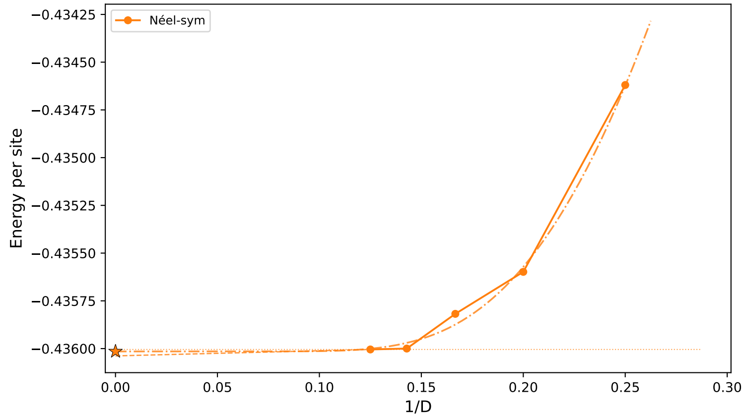
J_2=0.25 - Energy vs 1/D (Néel-sym) (dotted=horizontal, dashed=linear last-2, dash-dot=exp all- D s, ★= E_0 )
