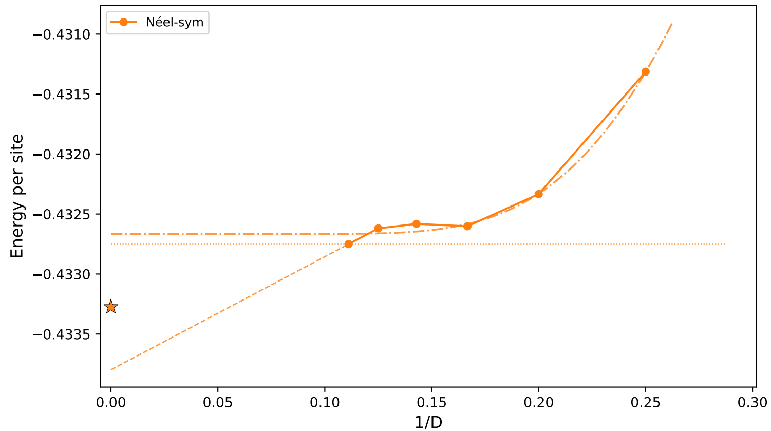
J_2=0.26 - Energy vs 1/D (Néel-sym) (dotted=horizontal, dashed=linear last-2, dash-dot=exp all- D s, ★= E_0 )
