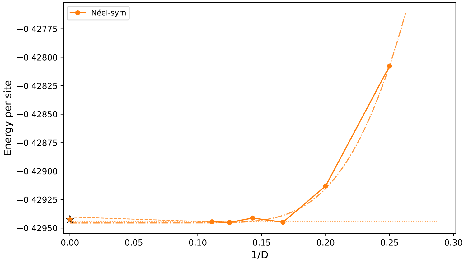
J_2=0.27 - Energy vs 1/D (Néel-sym) (dotted=horizontal, dashed=linear last-2, dash-dot=exp all- D s, ★= E_0 )
