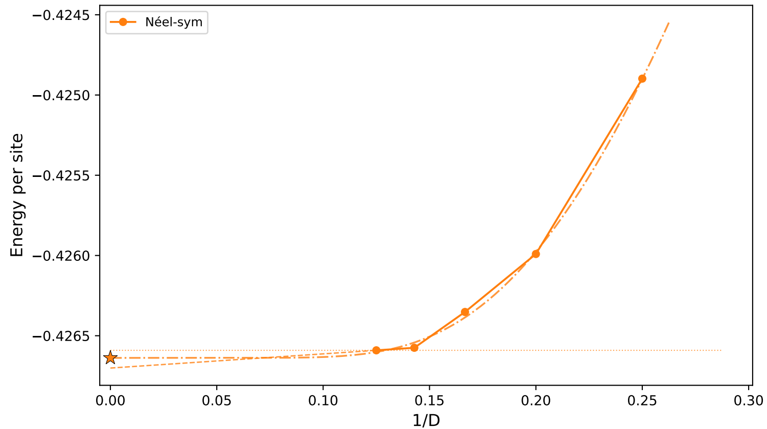
J_2=0.28 - Energy vs 1/D (Néel-sym) (dotted=horizontal, dashed=linear last-2, dash-dot=exp all- D s, ★= E_0 )
