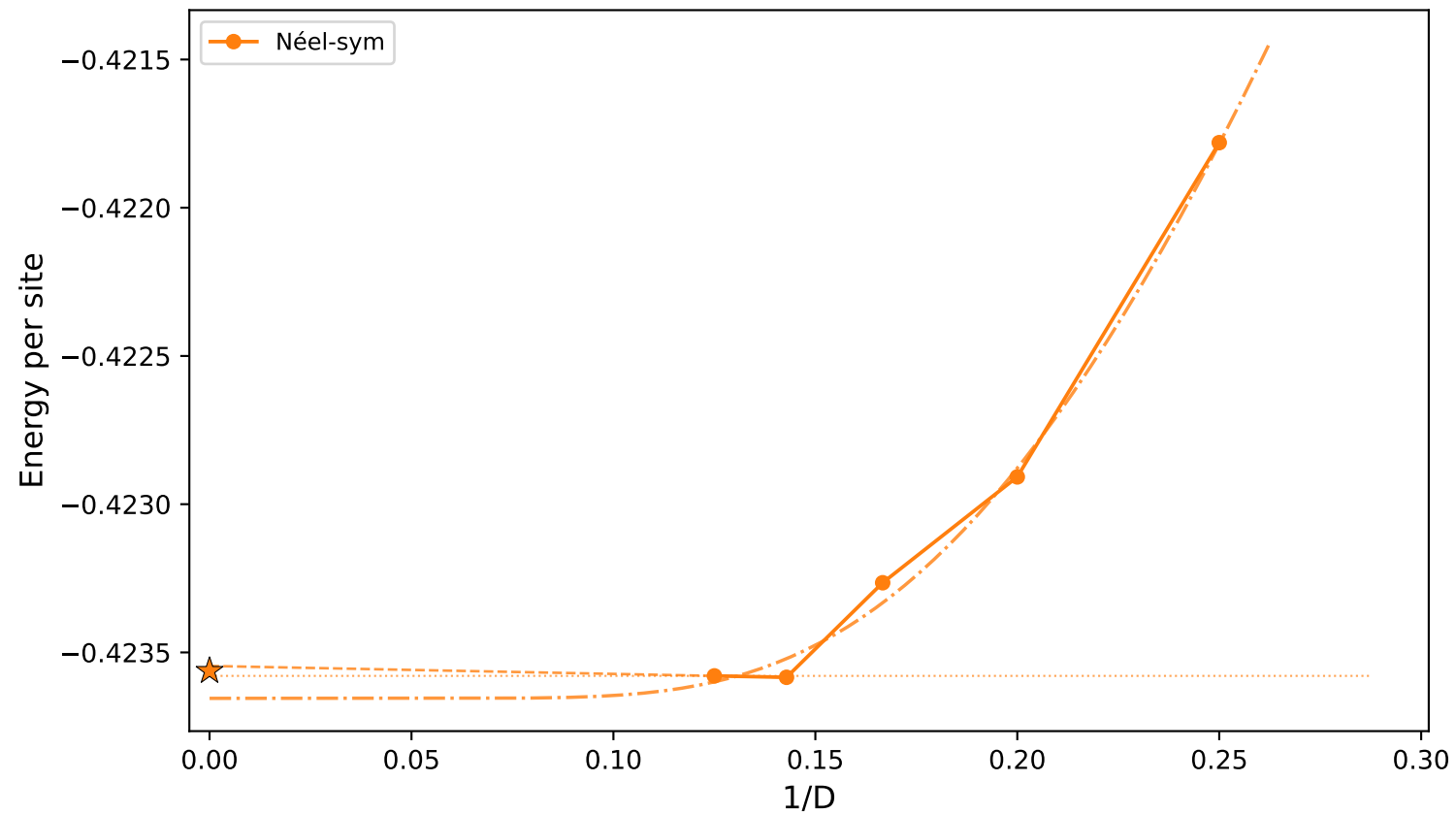
J_2=0.29 - Energy vs 1/D (Néel-sym) (dotted=horizontal, dashed=linear last-2, dash-dot=exp all- D s, ★= E_0 )
