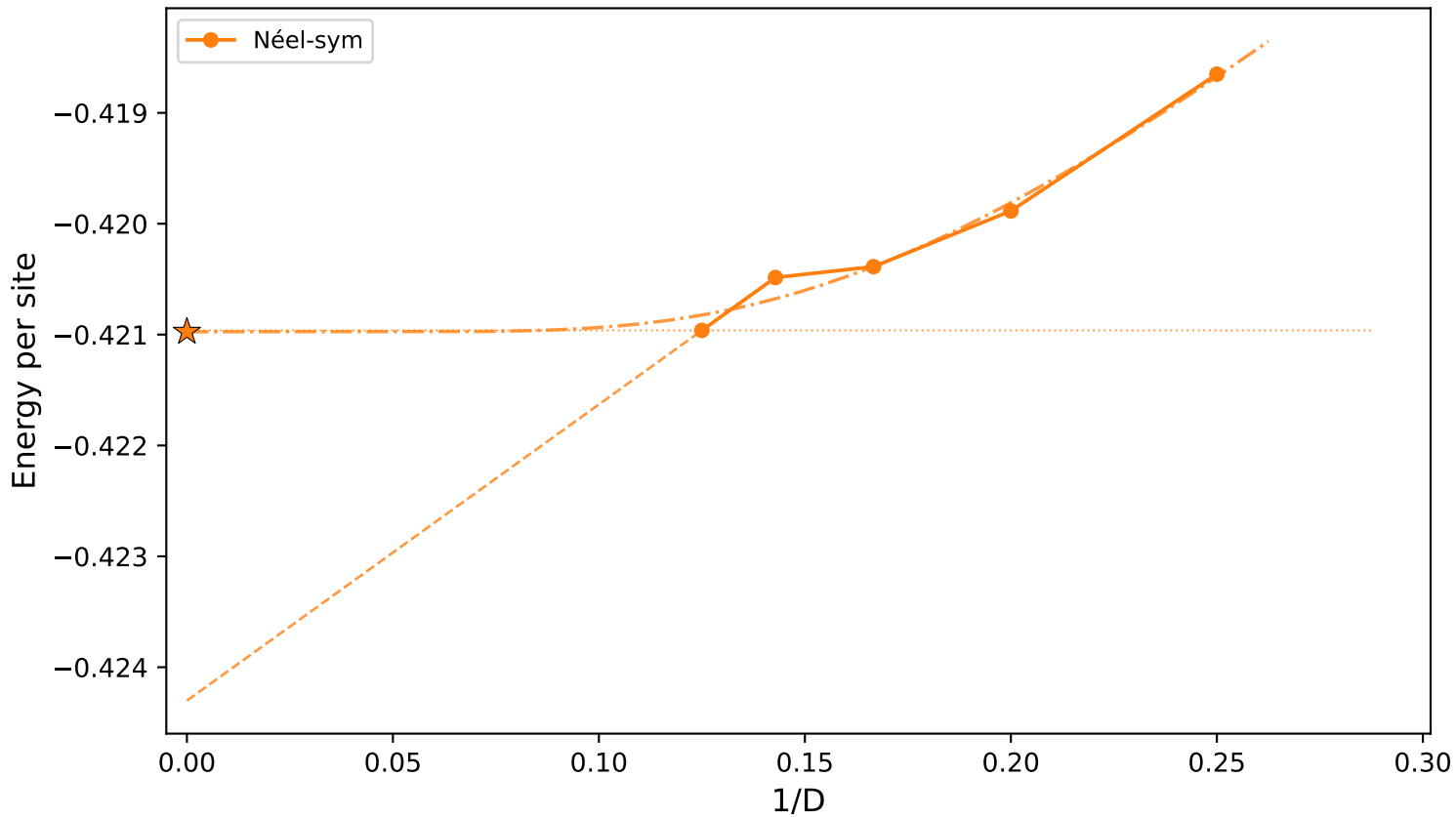
J_2=0.30 - Energy vs 1/D (Néel-sym) (dotted=horizontal, dashed=linear last-2, dash-dot=exp all- D s, ★= E_0 )
