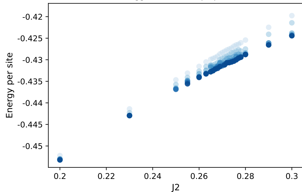
6-tensor (bigger D = more opaque & darker)
