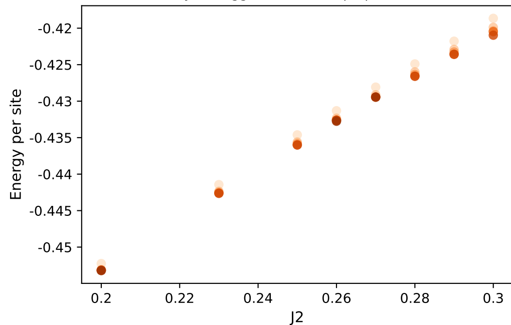
Néel-sym (bigger D = more opaque & darker)
