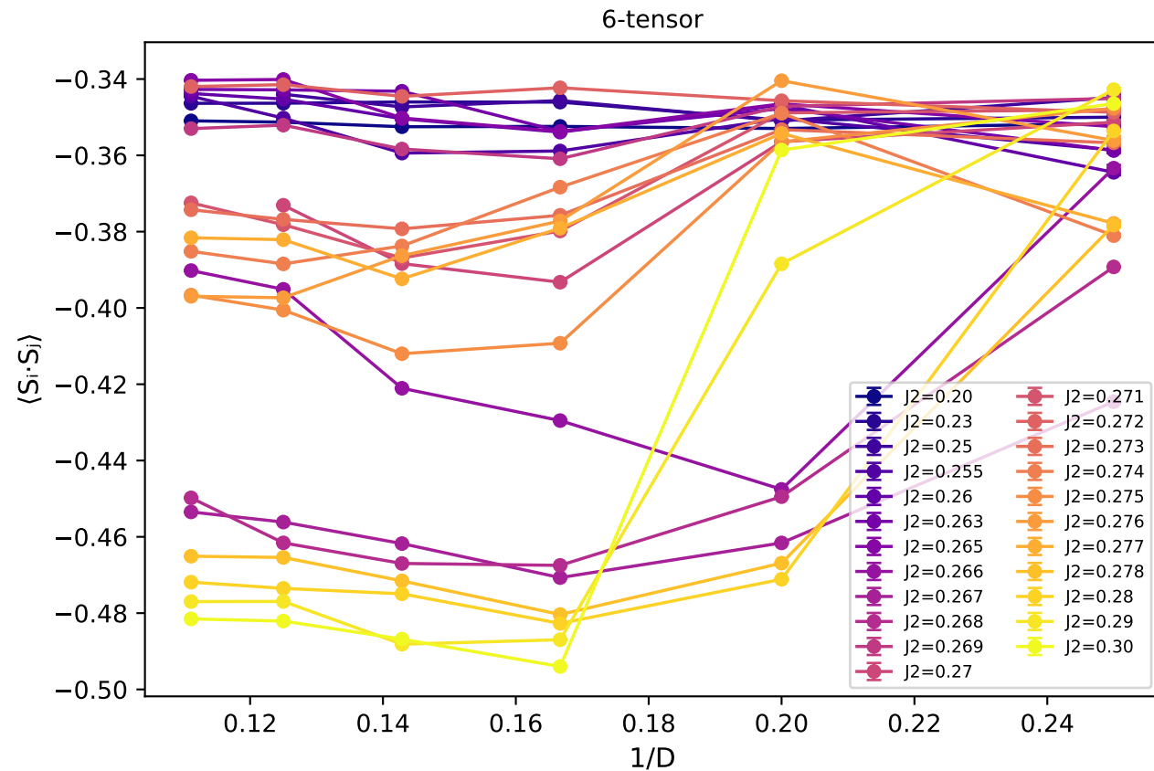
NN bond \langle S_i \cdot S_j \rangle - rank 1 group vs 1/D
