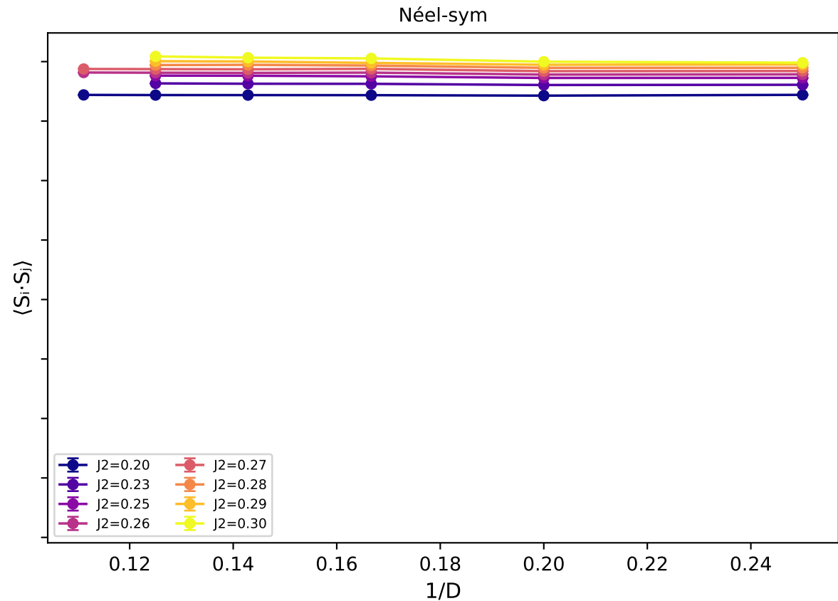
NN bond \langle S_i \cdot S_j \rangle - rank 1 group vs 1/D
