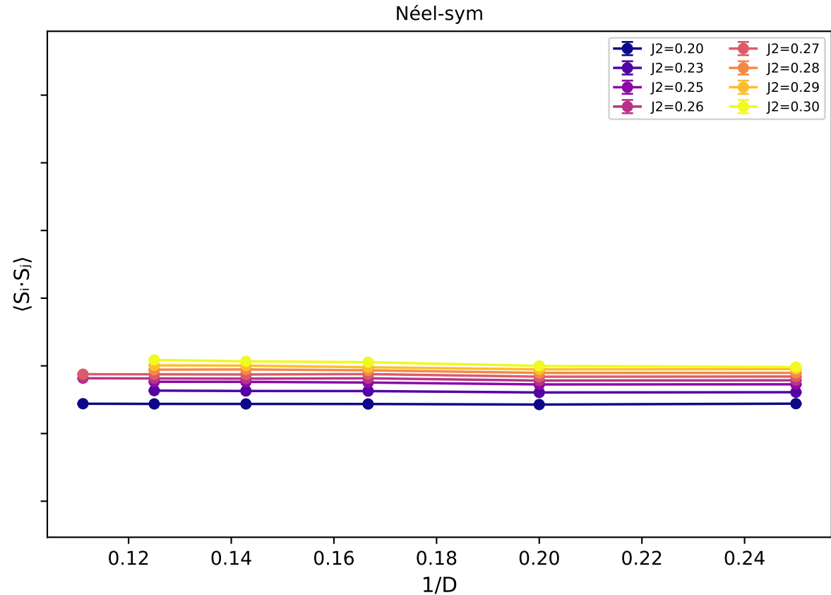
NN bond \langle S_i \cdot S_j \rangle - rank 2 group vs 1/D
