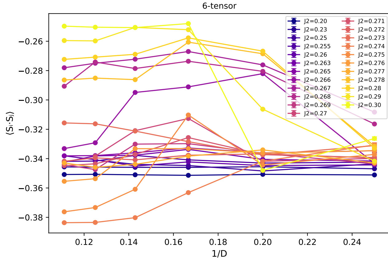
NN bond \langle S_i \cdot S_j \rangle - rank 2 group vs 1/D
