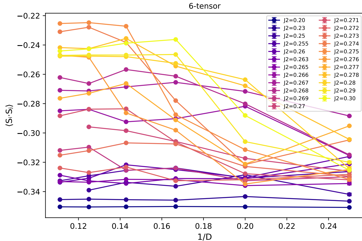
NN bond \langle S_i \cdot S_j \rangle - rank 3 group vs 1/D
