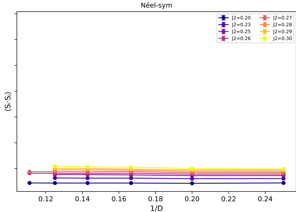
NN bond \langle S_i \cdot S_j \rangle - rank 3 group vs 1/D
