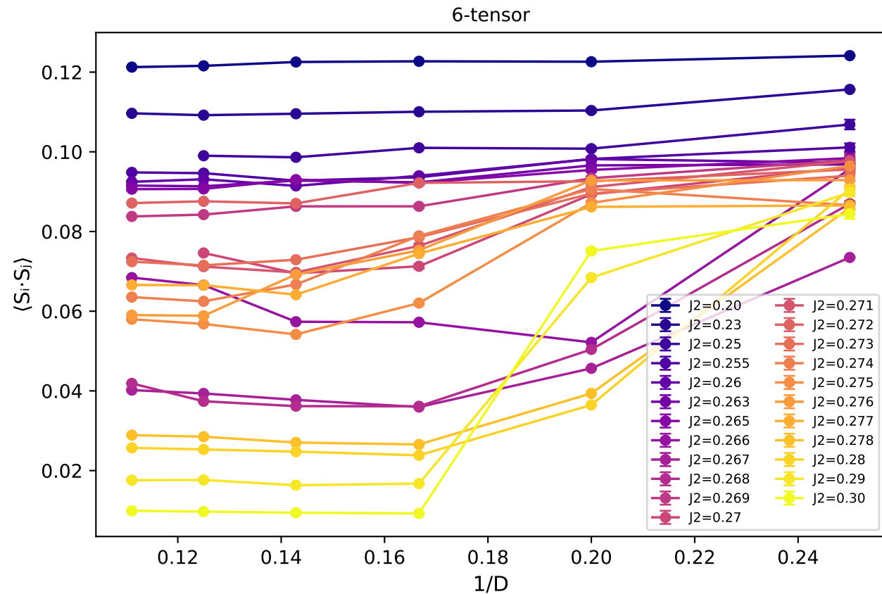
NNN bond \langle S_i \cdot S_j \rangle - rank 1 group vs 1/D
