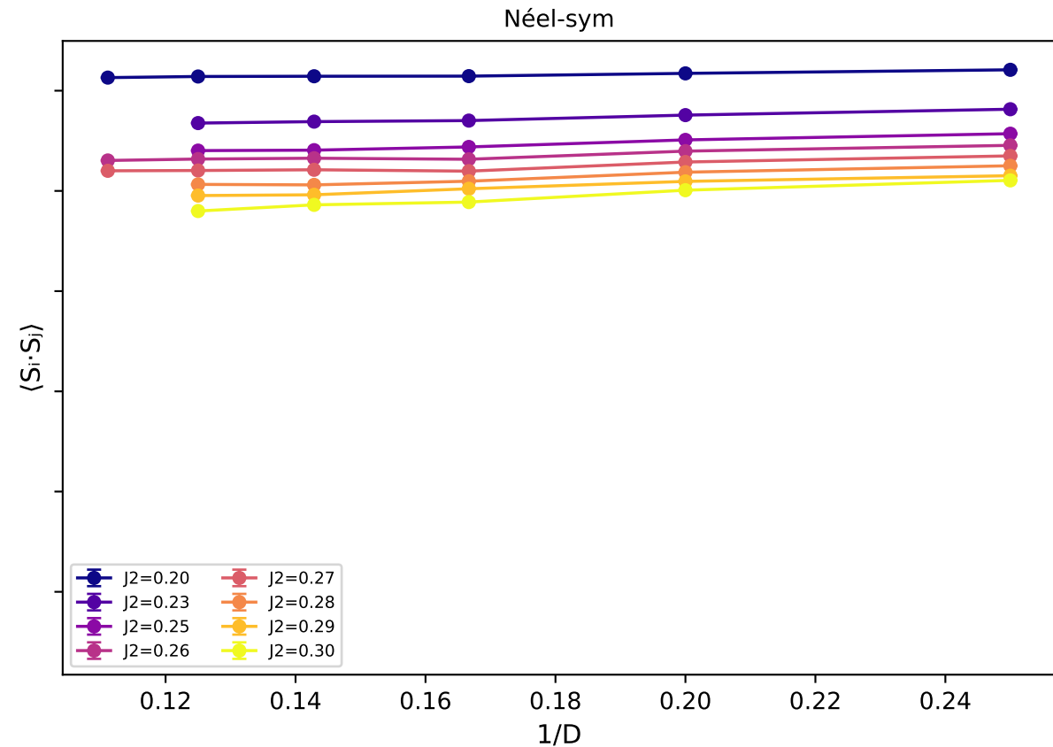
NNN bond \langle S_i \cdot S_j \rangle - rank 1 group vs 1/D
