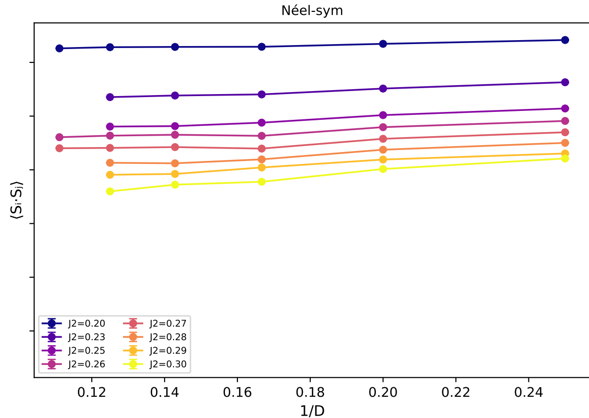
NNN bond \langle S_i \cdot S_j \rangle - rank 2 group vs 1/D
