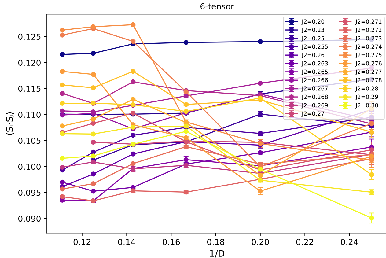
NNN bond \langle S_i \cdot S_j \rangle - rank 3 group vs 1/D
