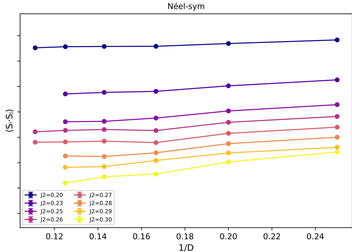
NNN bond \langle S_i \cdot S_j \rangle - rank 3 group vs 1/D
