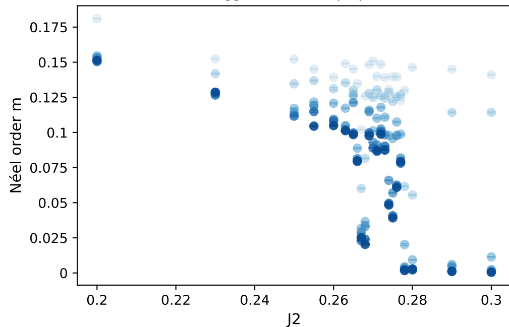
6-tensor (bigger D = more opaque & darker)
