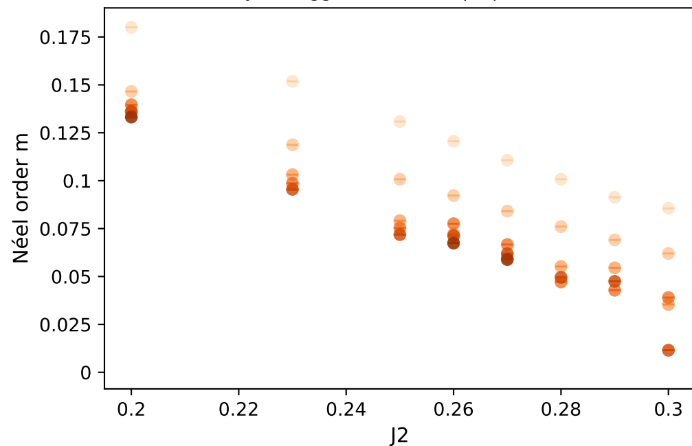
Néel-sym (bigger D = more opaque & darker)
