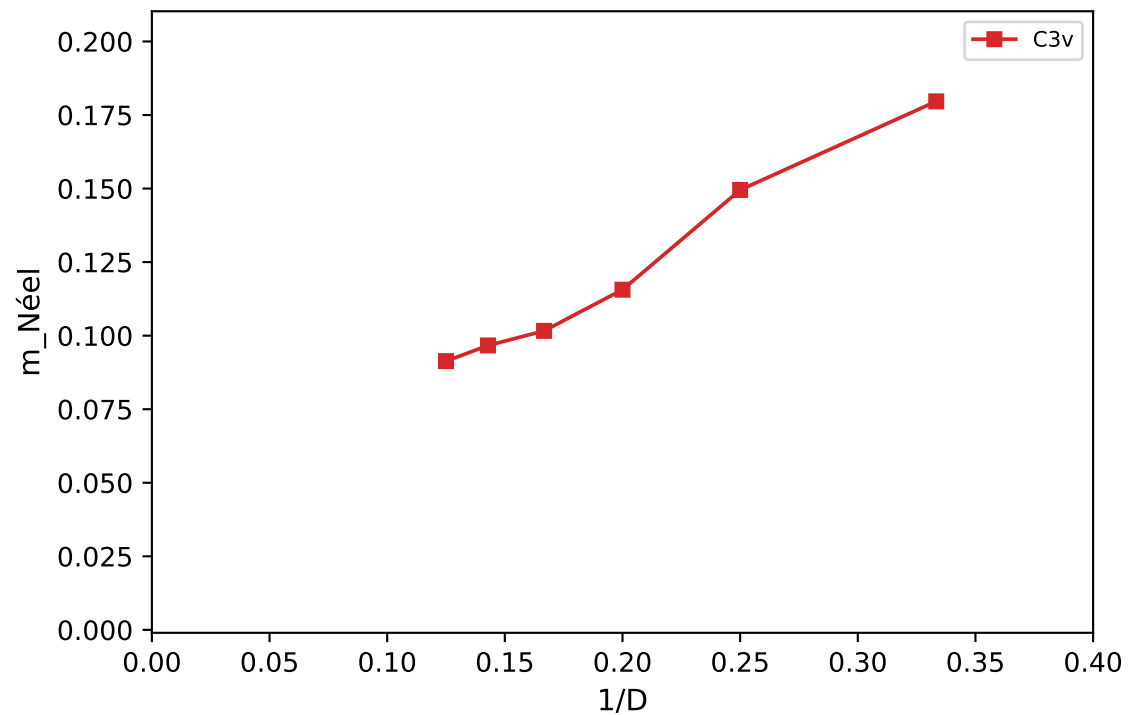
C3v
