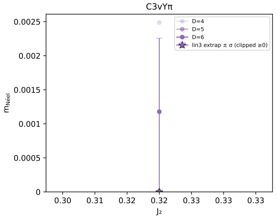
m_{\text{Néel}} vs J_2 — combined
