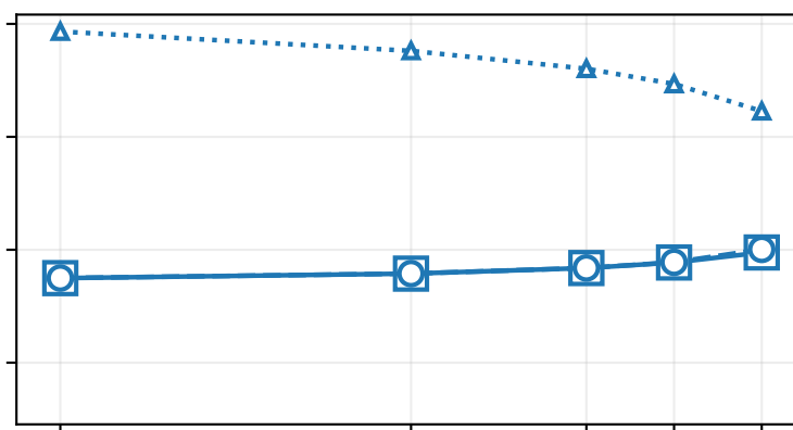
Plaquette pin
