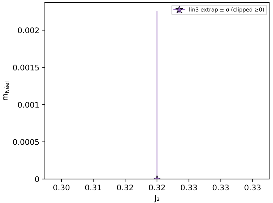
C3vY \pi
