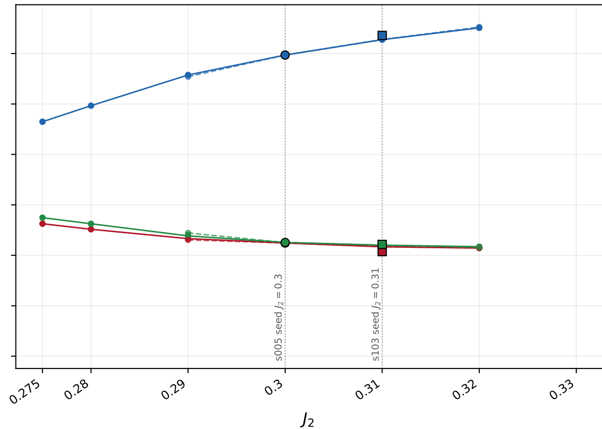
Plaquette seed, D = 9
