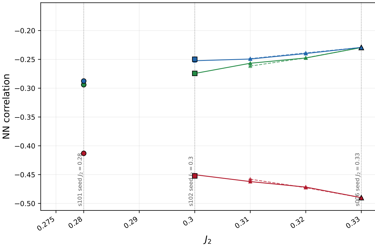
Dimer-plaquette seed, D = 9
